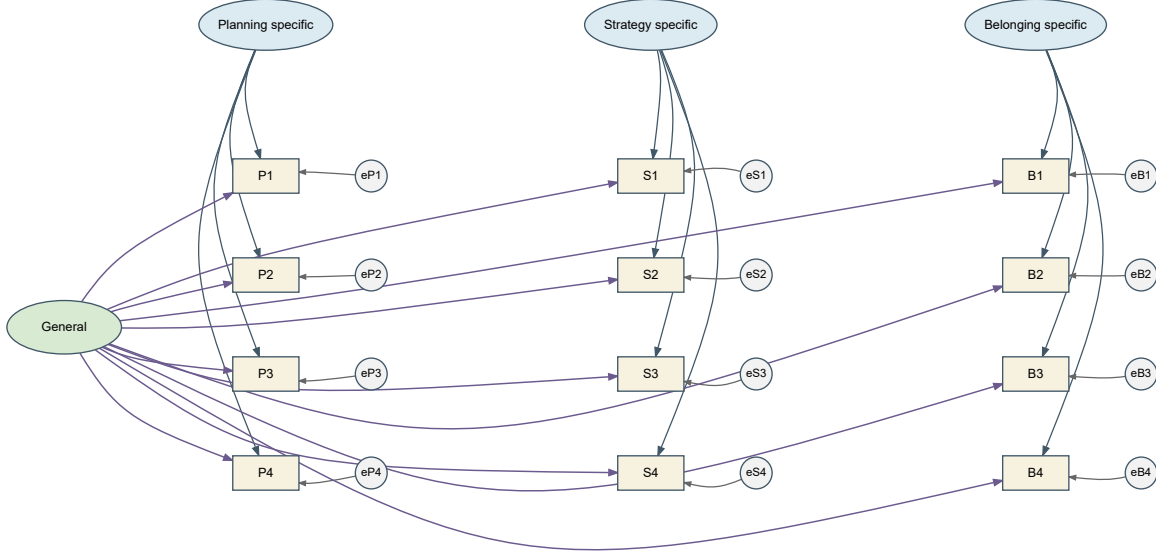
Figure 5: Orthogonal SLE bifactor model. General and the three domain-specific factors load directly on items; all four factors are mutually orthogonal and unshown loadings are zero.
