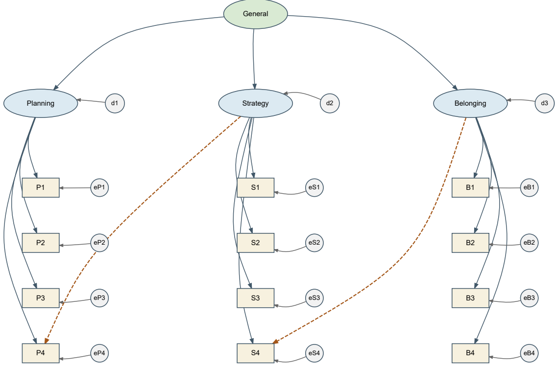
Figure 4: Higher-order representation of the inherited SLE measurement model. General accounts for first-order factor covariances; first-order disturbances remain, and the P4-on-Strategy and S4-on-Belonging loadings are retained.
