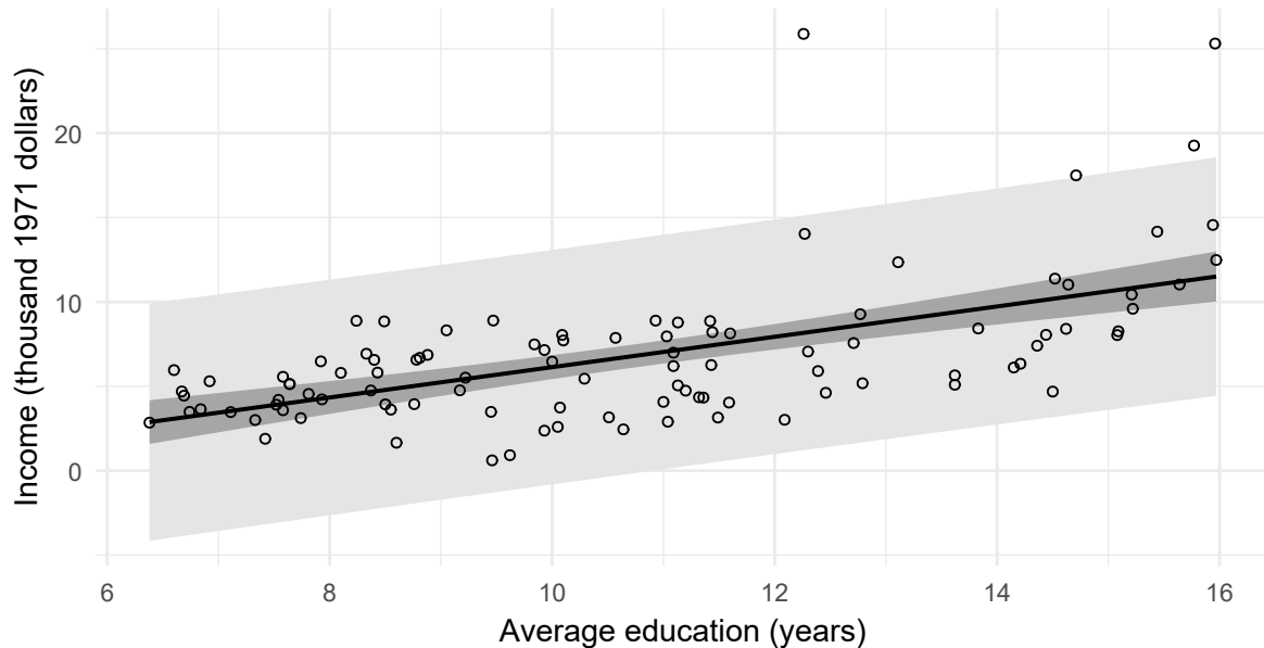
Figure 8: Confidence intervals for the mean response (dark band) and prediction intervals for one new occupation (light band), from the same fitted line.
