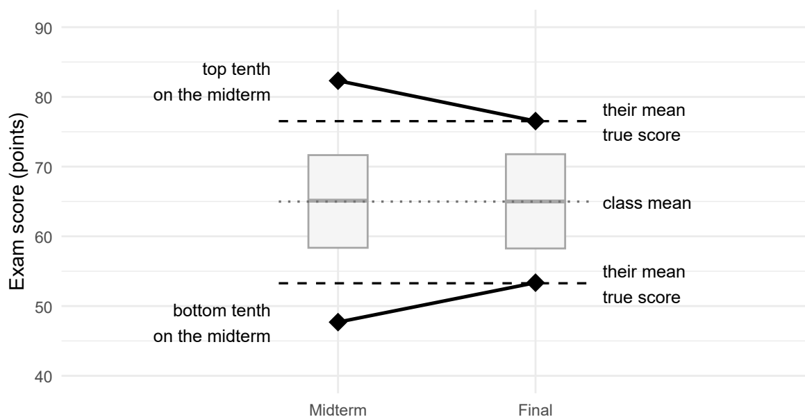
Figure 12: A hypothetical class of 2,000 students, each score a stable true score plus independent luck. The top and bottom tenth on the midterm (diamonds) score nearer the class mean on the final, at their unchanged mean true score (dashed); the boxes, the middle half of the class, span about the same range of scores on the final as on the midterm.
