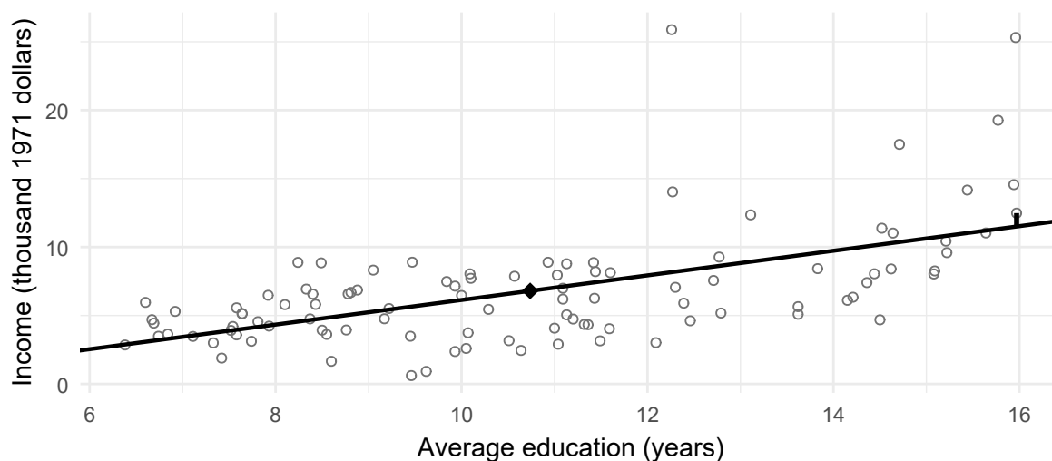
Figure 2: The least-squares line passes through the mean point; the marked vertical segment is the university-teacher residual.
