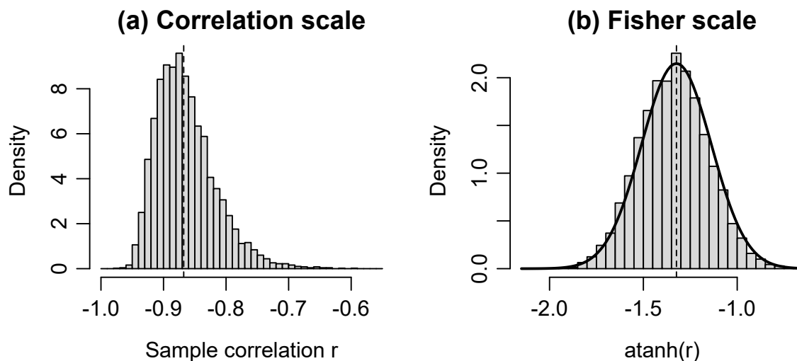
Figure 15: Sample correlations from 5,000 simulated studies of 32 pairs with process correlation -.8677 . (a) On the correlation scale the distribution is skewed, with a long tail toward zero and a hard limit at -1 ; (b) on the Fisher scale it is nearly Normal, and the curve is the Normal density with SD 1/\sqrt{29} . Dashed lines mark the process value on each scale.
