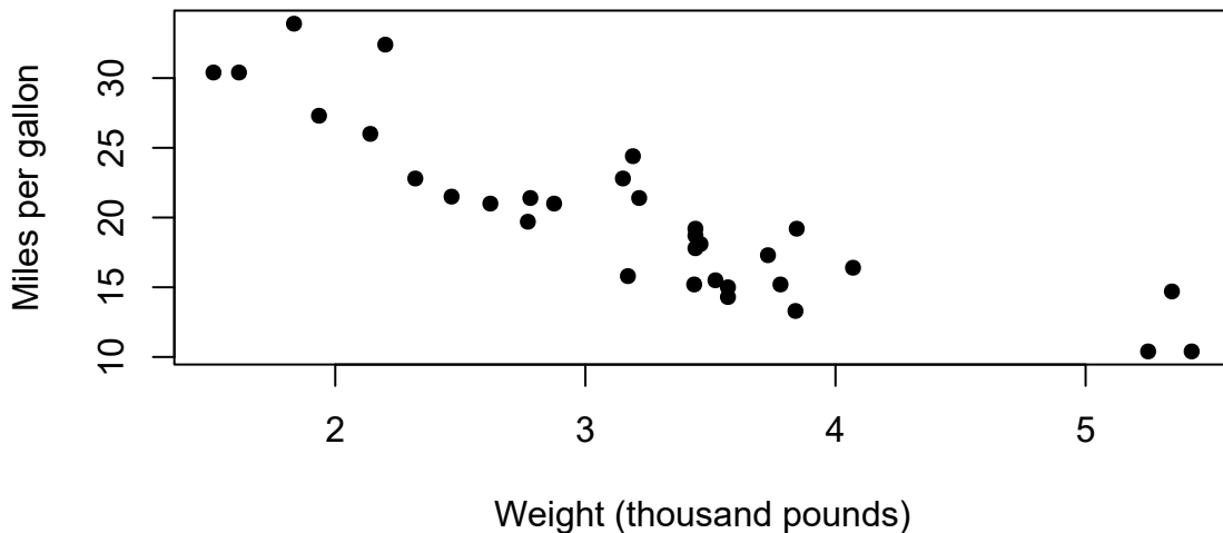
Figure 5: Mileage and weight for 32 recorded car models.
