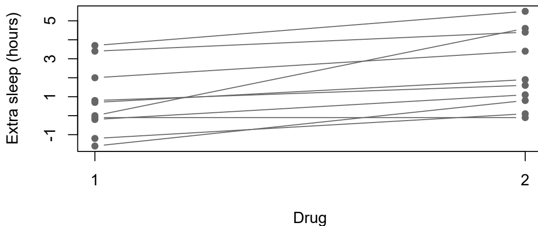
Figure 13: Two measurements for each of ten people.
