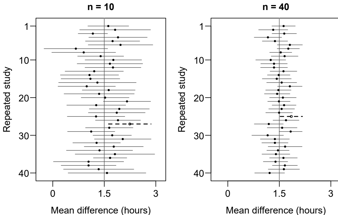
Figure 14: Fresh data produce different 95% t intervals. Each dot is a sample mean, and its segment uses that study's estimated SE. The vertical line is the fixed true mean, 1.5 hours; dashed segments and open dots mark intervals that miss it. Each panel shows the first 40 of the corresponding table's 2,000 studies, with seed 60610 reset for each sample size. In each panel, 39 of 40 intervals cover.
