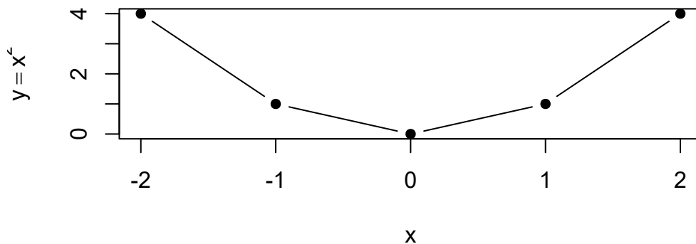
Figure 6: An exact curved relationship with zero Pearson correlation.
