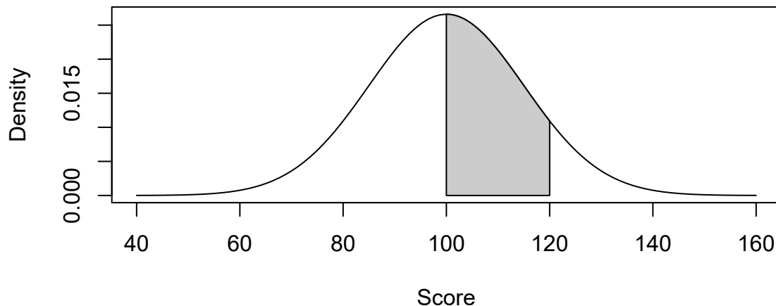
Figure 3: Probability is an area under a stipulated Normal density.
