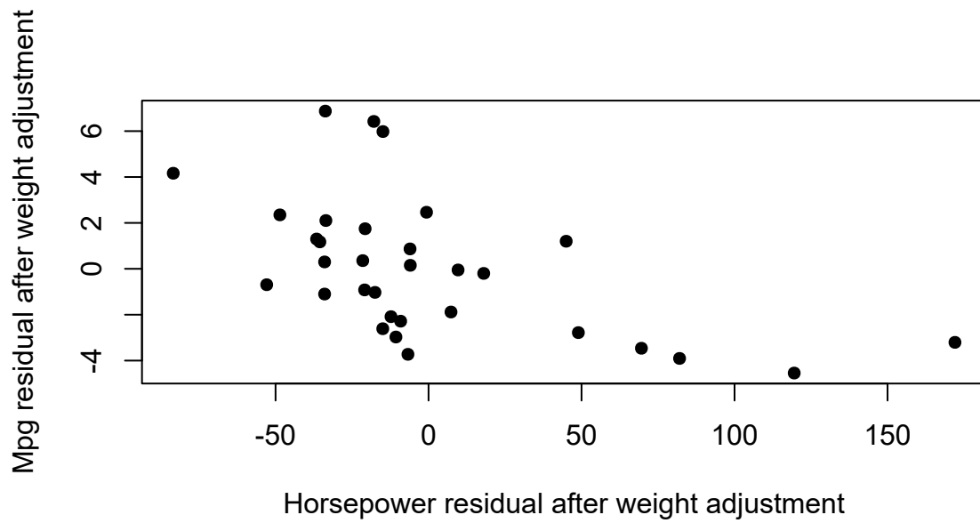
Figure 9: Mileage and horsepower after separately fitting their linear relationships with weight.
