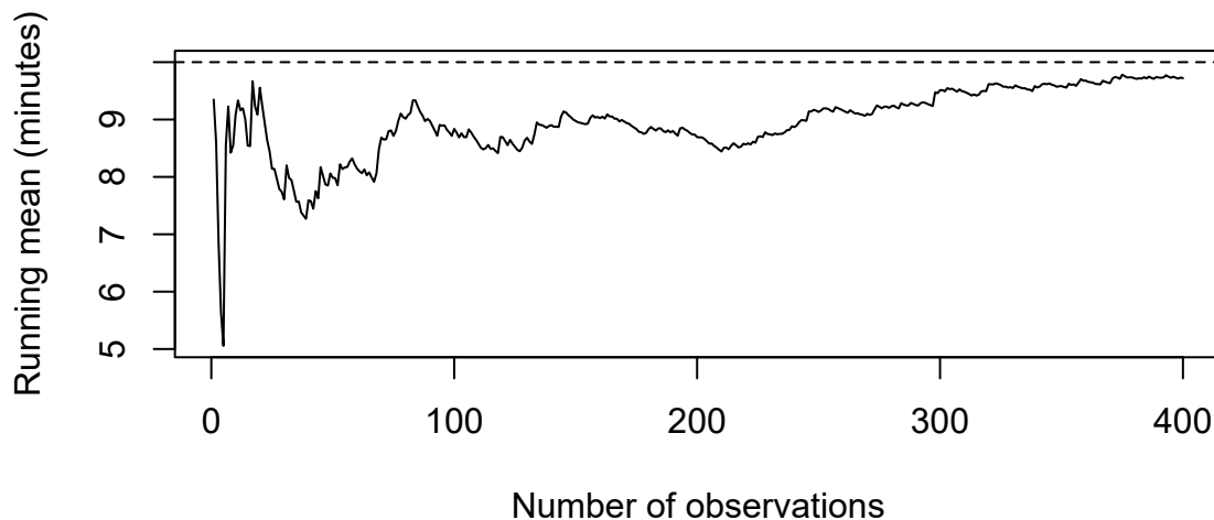
Figure 11: One running mean from independent exponential waits with model mean ten minutes.
