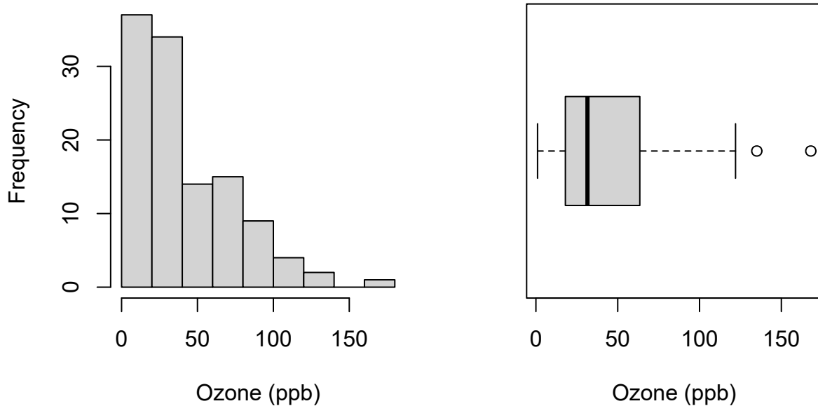
Figure 1: Recorded ozone values on 116 days, displayed as a histogram and a boxplot.
