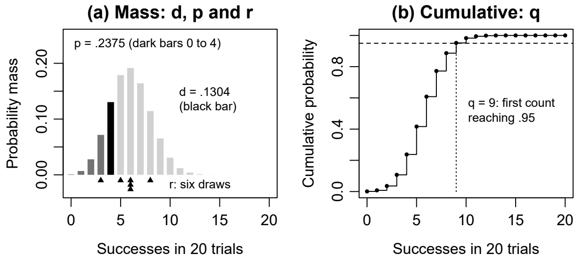
Figure 4: Four questions asked of one binomial model, 20 trials with success probability .3. (a) The mass at 4 (black bar) is what dbinom returns; the masses at 0 to 4 together (dark bars) are what pbinom returns; the triangles below the axis are the six counts from rbinom . (b) The cumulative probability first reaches .95 at 9, the value qbinom returns.
