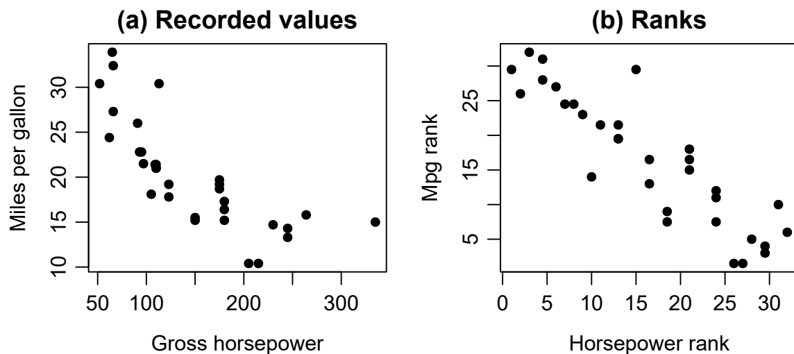
Figure 8: Mileage and horsepower for the 32 models, (a) on the recorded scales and (b) as ranks. The curved decline in (a) weakens the linear coefficient; ranks straighten a monotone pattern.
