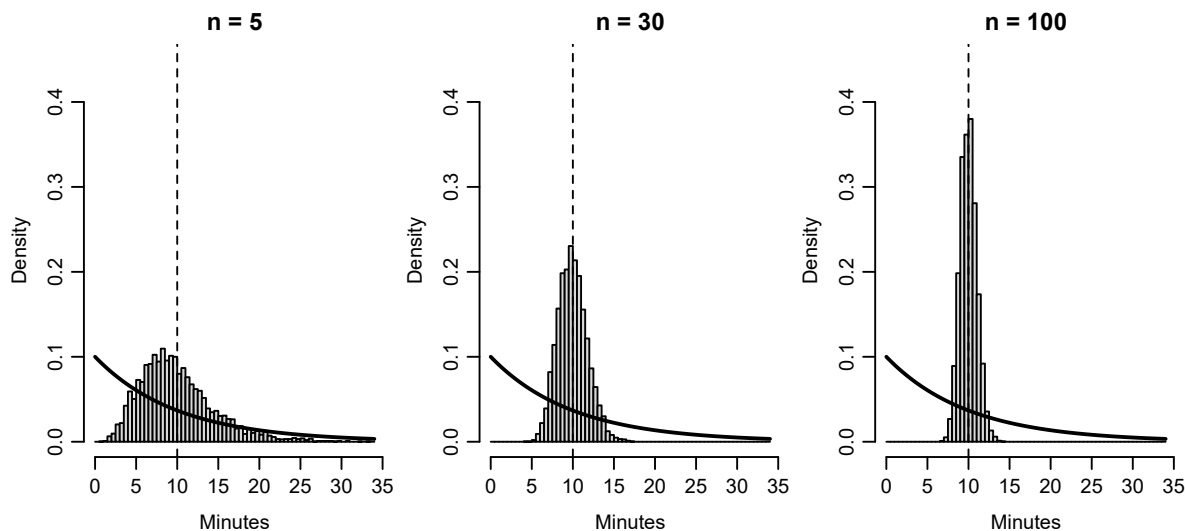
Figure 12: Individual waits and averages answer different questions. The line in every panel is the same exponential density for a single wait, with mean and SD ten minutes. Histograms show 5,000 independent sample means at each sample size. The dashed line marks their common model mean.
