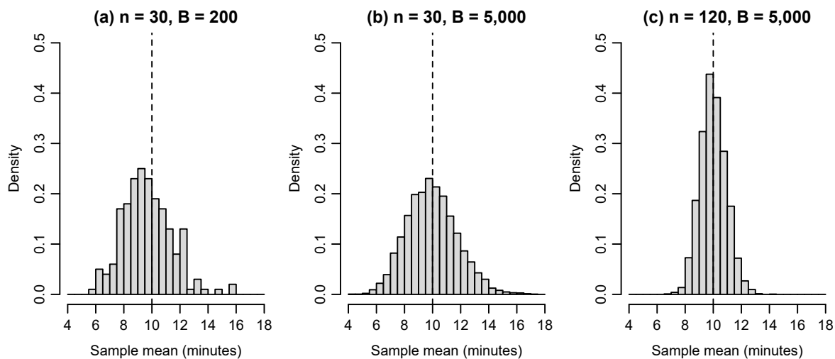
Figure 10: More repetitions or larger studies. Each histogram collects simulated sample means from the waiting-time model; the dashed line marks the model mean, 10 minutes. (a) The first 200 of the 5,000 means of 30 waits; (b) all 5,000; (c) 5,000 means of 120 waits.
