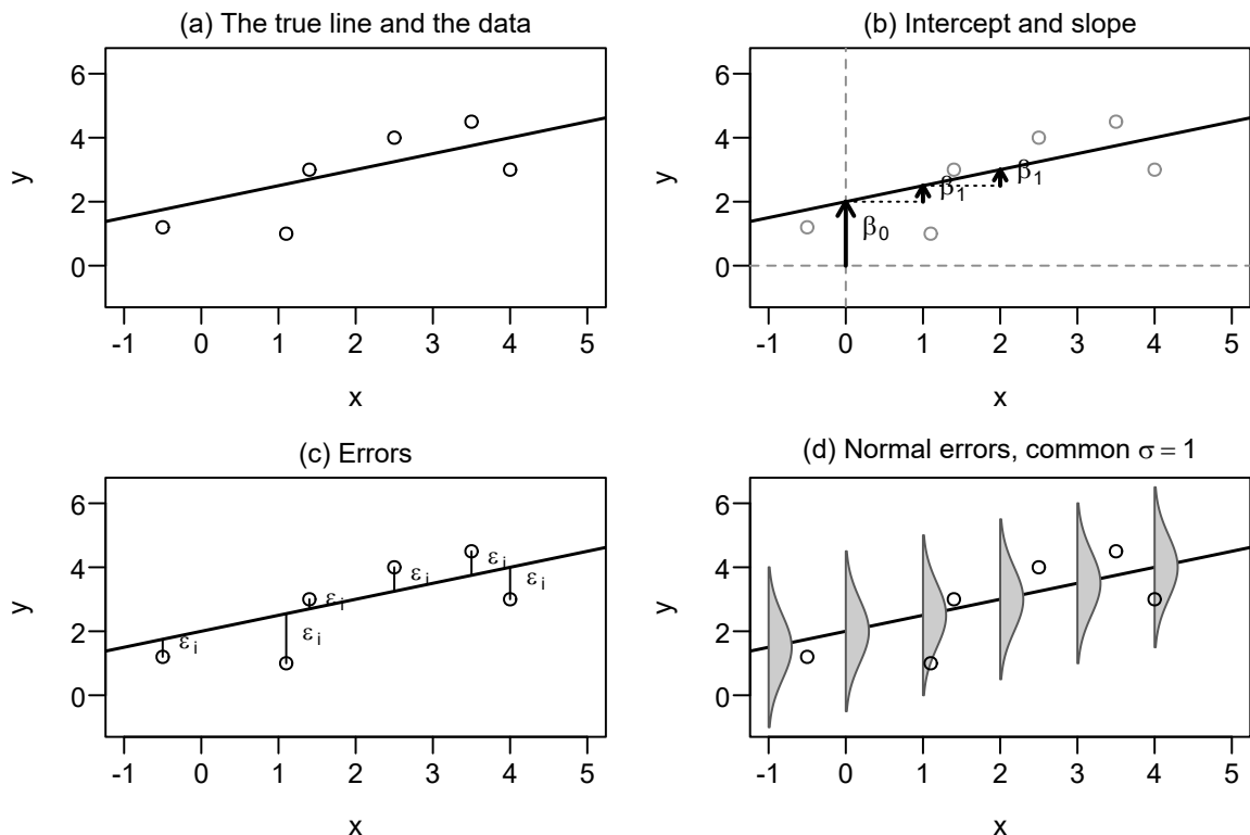
Figure 1: The parts of the simple regression model, drawn on six invented points around the true line y = 2 + 0.5x . (a) The true line and the data. (b) The intercept \beta_0 is the mean of y at x = 0 , and the slope \beta_1 is the difference in mean y for a one-unit difference in x . (c) The errors \varepsilon_i are the vertical distances from the points to the true line. (d) The errors follow one Normal distribution around the line, with the same SD, here \sigma = 1 , at every x .
