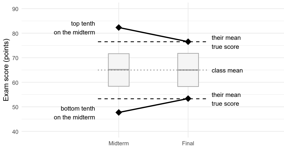
Figure 13: A hypothetical class of 2,000 students, each score a stable true score plus independent luck. The top and bottom tenth on the midterm (diamonds) score nearer the class mean on the final, near their unchanged mean true score (dashed); the boxes, the middle half of the class, span about the same range of scores on the final as on the midterm.
