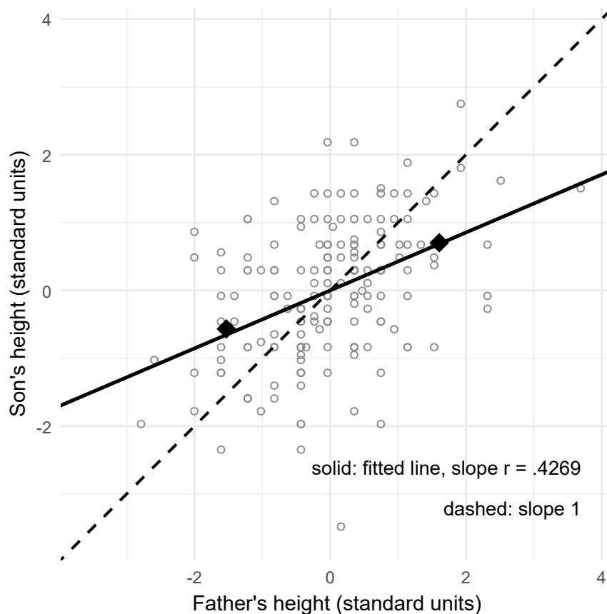
Figure 12: Galton's 179 fathers and sons in standard units. The fitted line has slope r = .4269 , flatter than the dashed line of slope 1; the filled points are the mean positions of the fathers more than 1 SD above and below their mean, with their sons.
