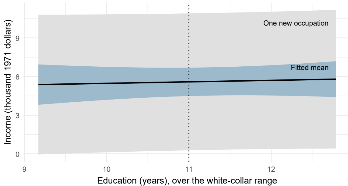
Figure 7: Two 95% intervals for a white-collar profile at prestige 45 and women 50, across the white-collar education range.
