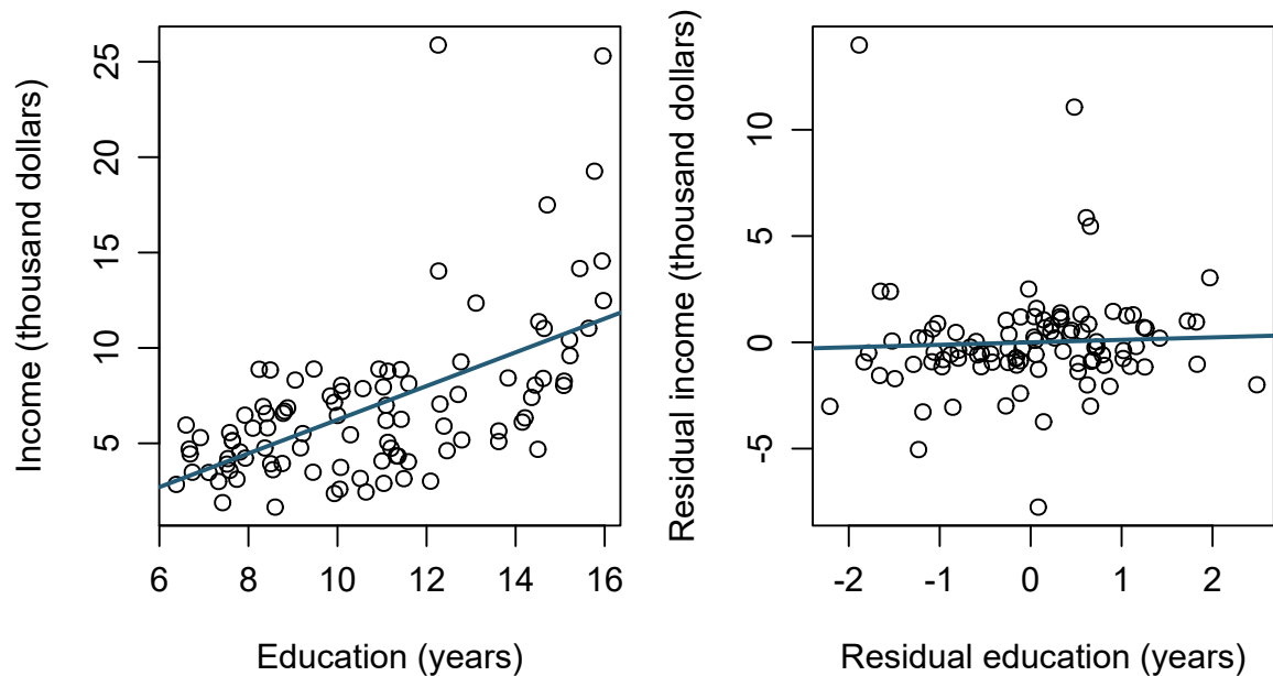
Figure 3: Marginal and residualized income–education comparisons in the same 98 occupations.
