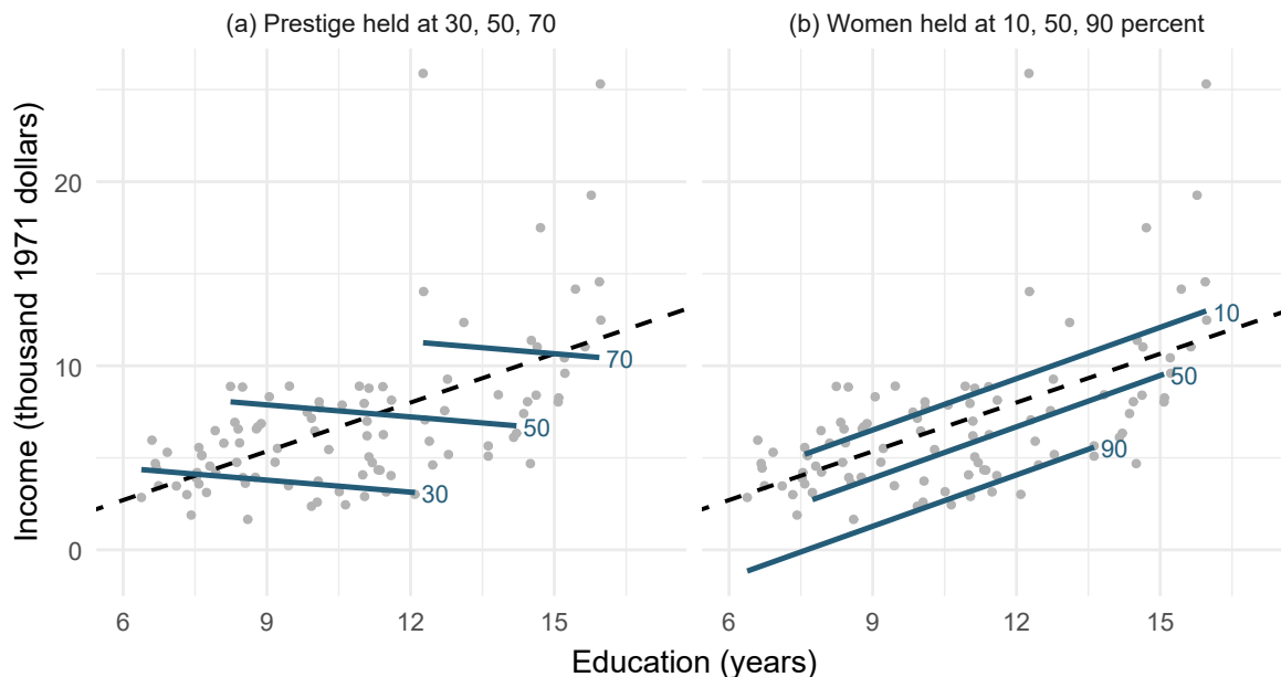
Figure 2: Fitted income against education at three held values of prestige (a) or of the percentage of women (b), each line drawn over the education observed near its held value, with the dashed marginal education-only line.
