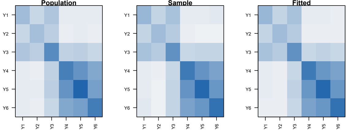
Figure 3: Known population, one sample and the correctly specified fitted covariance. All panels use the same indicator order and color scale; the selected entries below give the numerical comparisons. The third panel will be explained through estimation and evaluation.
