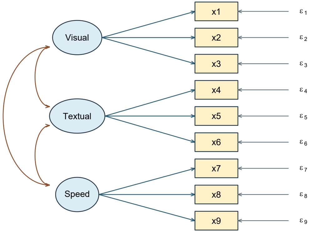
Figure 16: A declared three-factor model for the nine historical tests. Factor variances equal one, all three factor covariances are free, and unshown loadings and residual covariances are zero.
