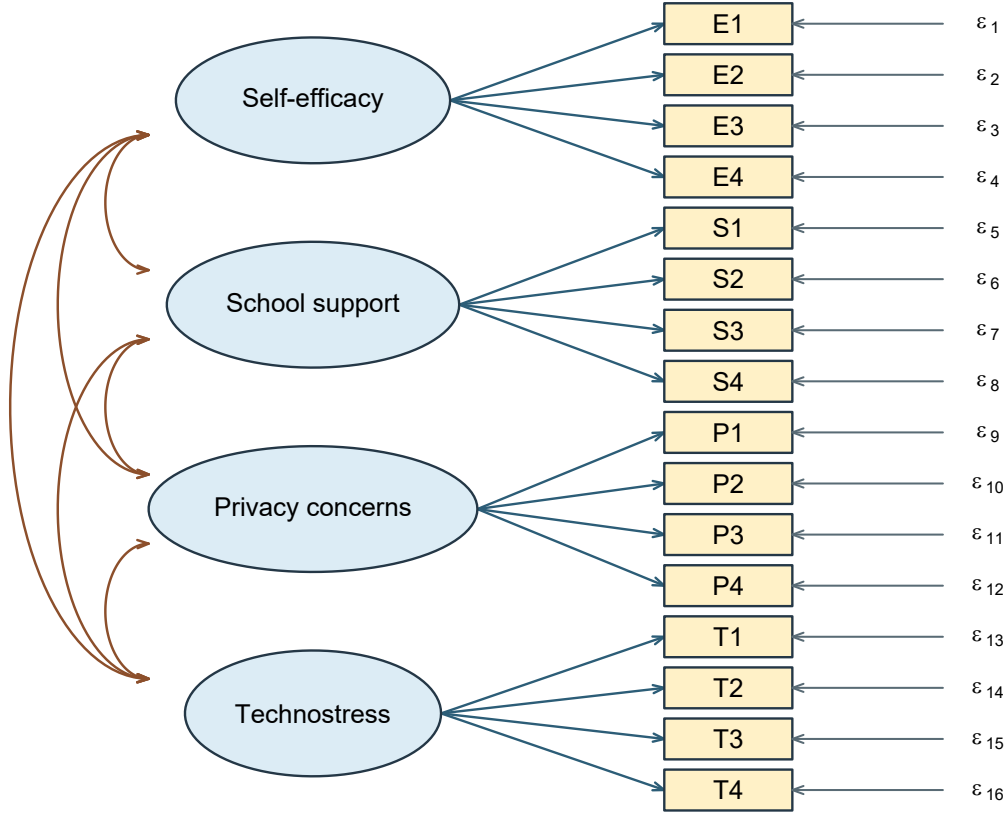
Figure 6: Four-factor, sixteen-indicator CFA reconstructed as a diagram-reading transfer. All six factor correlations are free; fixed-factor scaling is used for the count.
