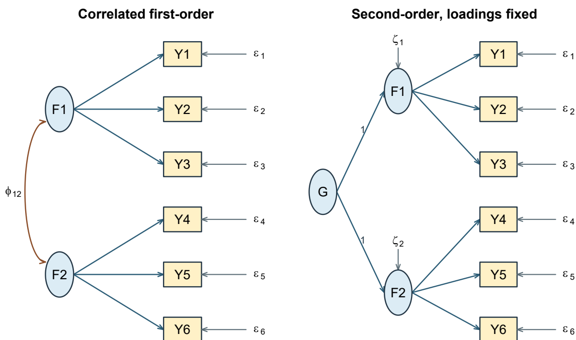
Figure 12: A correlated two-factor model and one constrained second-order reparameterization. The equivalence requires the stated fixed loadings and admissible disturbance variances.
