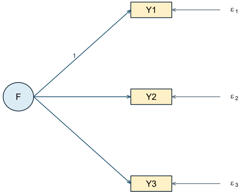
Figure 9: A marker-scaled three-indicator block. The three off-diagonal covariances can recover the factor variance and two non-marker loadings at regular, nonzero parameter points.
