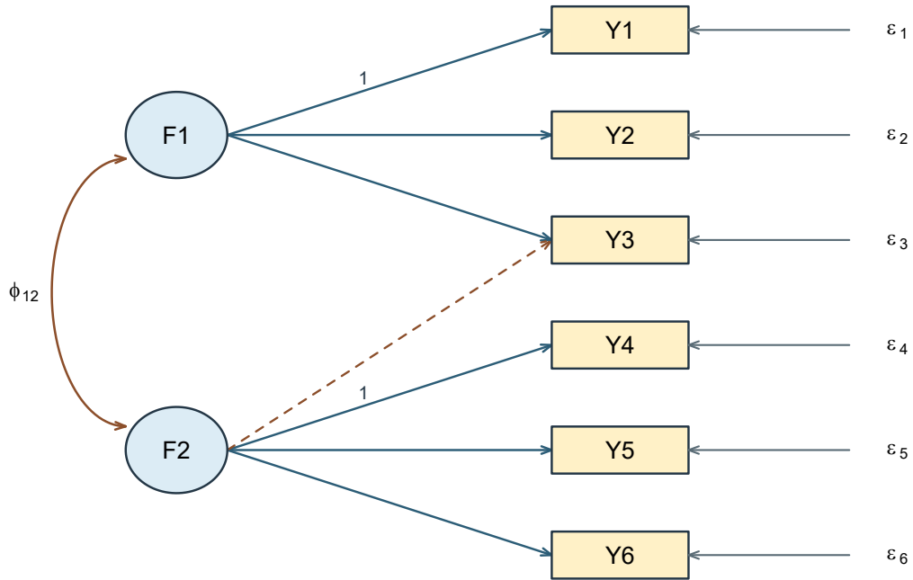
Figure 2: The disclosed generating model for the six-indicator simulation. Y_3 has two loadings. The Y_1 and Y_4 loadings equal one, setting the factor units. Residual covariances and unshown loadings are zero.
