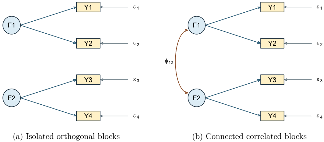
Figure 10: Both two-indicator models have positive nominal degrees of freedom, yet different recoverability. Adding the covariance edge increases the free-parameter count from eight to nine and supplies informative cross-block moments.
