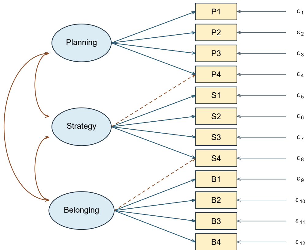
Figure 14: The exact M1-cross structure carried into evaluation, not a redrawn simple-structure substitute.
