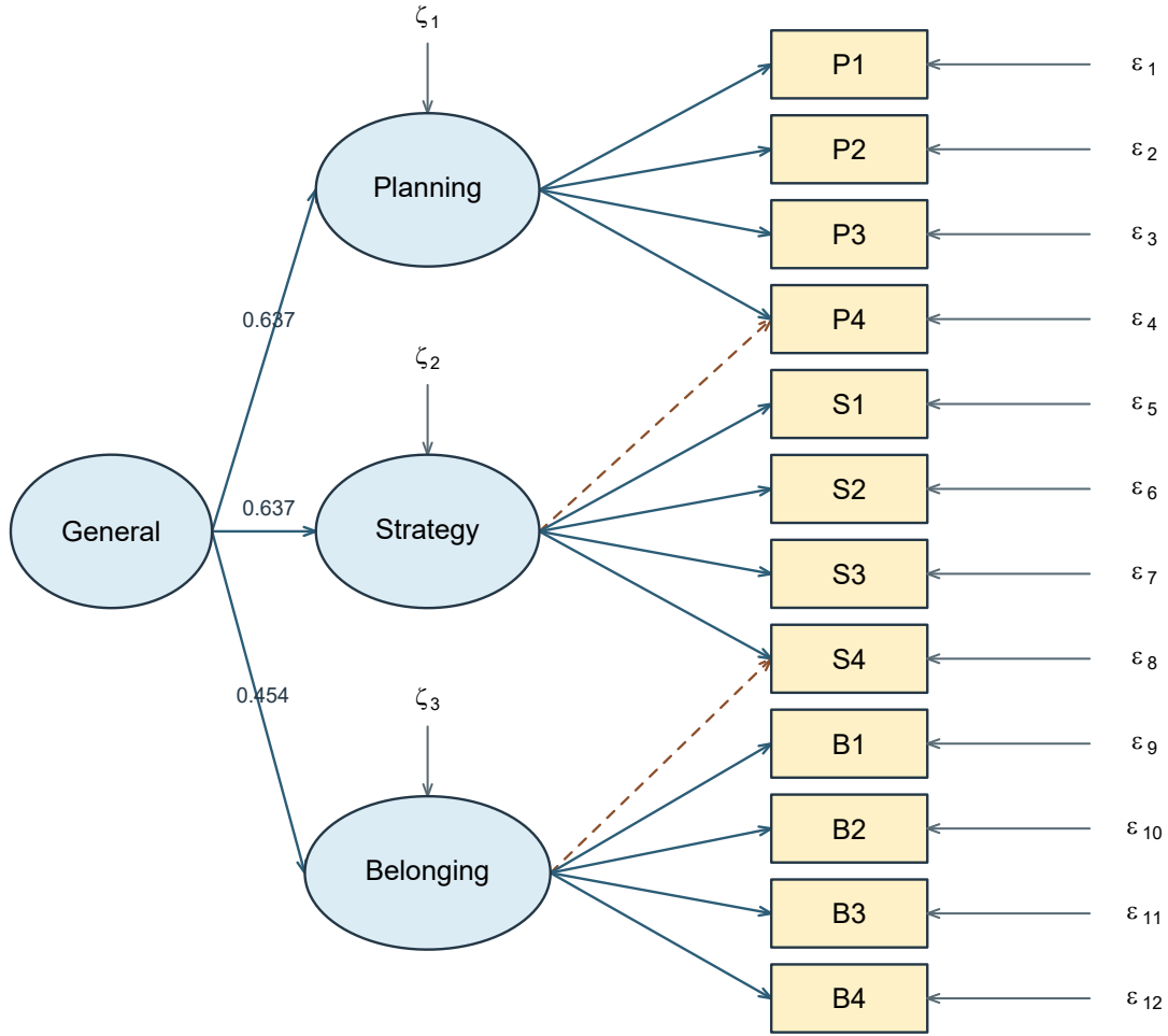
Figure 5: Higher-order representation of the inherited SLE measurement model. General accounts for first-order factor covariances; first-order disturbances remain, and the P4-on-Strategy and S4-on-Belonging loadings are retained.
