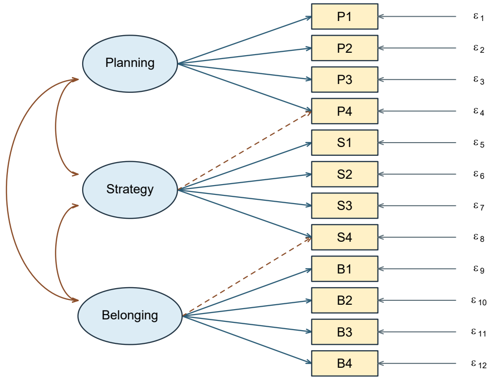
Figure 1: The fixed questionnaire model to be evaluated. Ovals are factors, boxes indicators, one-headed arrows loadings, curved two-headed arrows factor covariances, and the small residual terms supply indicator-specific variance. The two secondary loadings are part of the original candidate.
