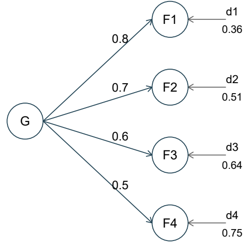
One higher-order factor
