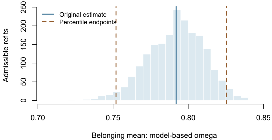
Figure 9: Belonging omega across 2,000 attempted and 2,000 admissible refits of fixed M1-cross. The solid line is the original estimate; dashed lines mark the percentile 95% interval. Every resample retains whole twelve-indicator records.
