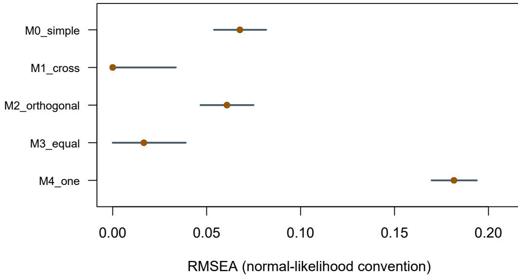
Figure 2: RMSEA point estimates and 90 percent intervals for the planned models. No traffic-light cutoffs are imposed.
