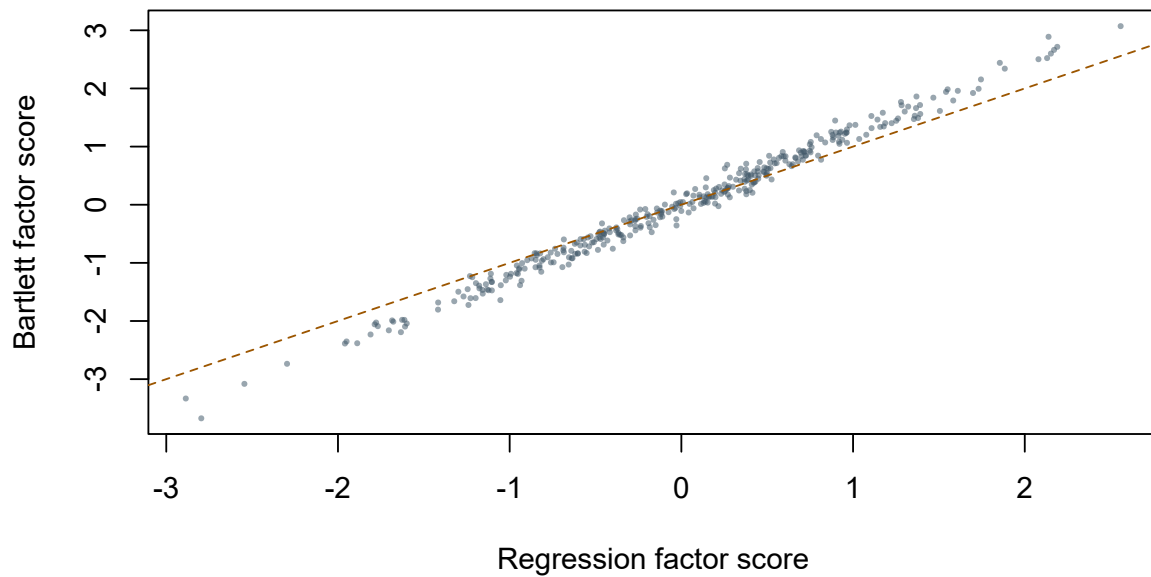
Figure 10: Two ways of scoring Planning in the same synthetic Sample B. Agreement is not identity and neither axis is an observed true factor value.
