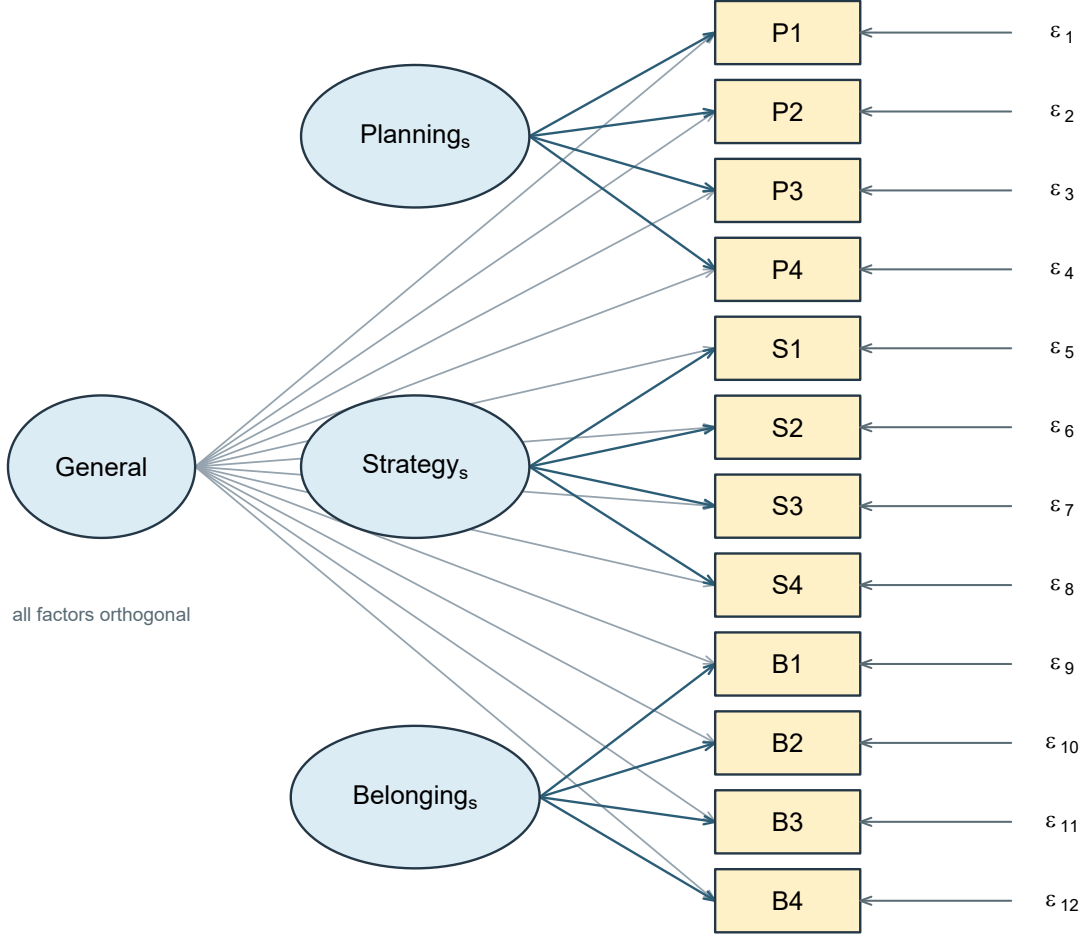
Figure 7: Orthogonal SLE bifactor model. General and the three domain-specific factors load directly on items; all four factors are mutually orthogonal and unshown loadings are zero.
