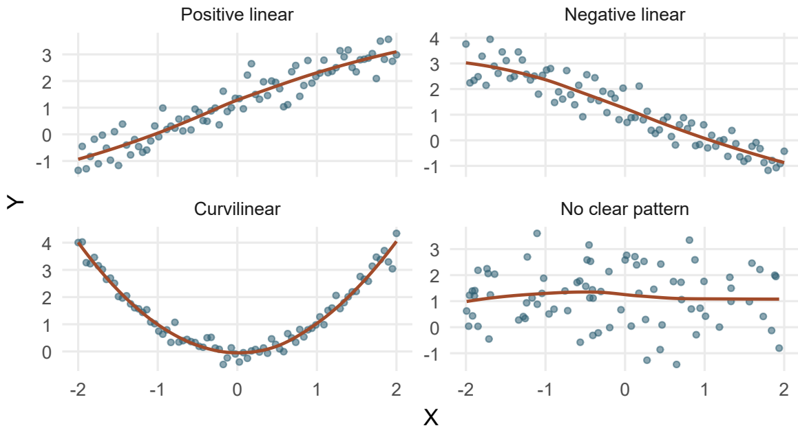
Figure 11: Linear, curvilinear, and patternless relationships require different descriptions.
