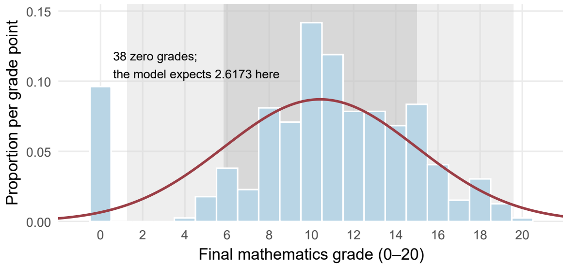
Figure 9: Checking a Normal model against the 395 final grades. The curve is the Normal density with the observed mean and SD; the darker band marks one SD and the lighter band two SDs on each side of the mean.
