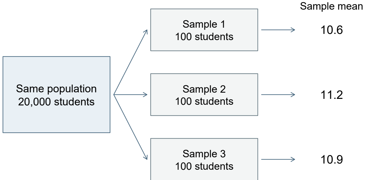
Figure 14: Repeating the same sampling process produces a distribution of sample means. The grade values are invented illustrations.
