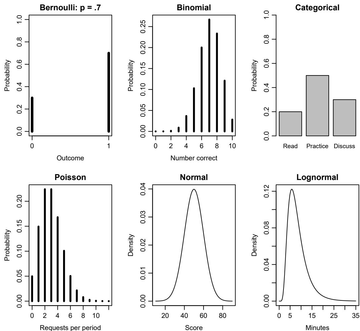
Figure 7: Six probability models with declared parameters: masses for discrete outcomes and density curves for continuous outcomes.
