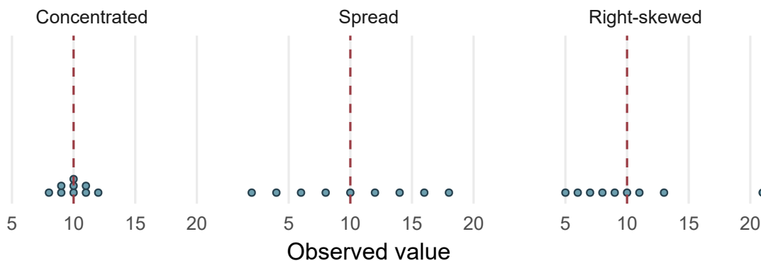
Figure 4: Three invented distributions share a mean of 10 but differ in shape and spread.
