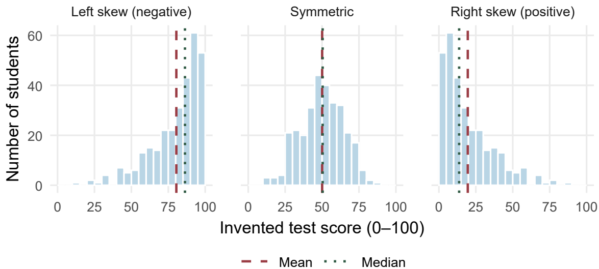
Figure 3: Three invented distributions of 300 test scores. The long tail names the direction of a skew, and the mean lies toward it; dashed and dotted lines mark the mean and median.
