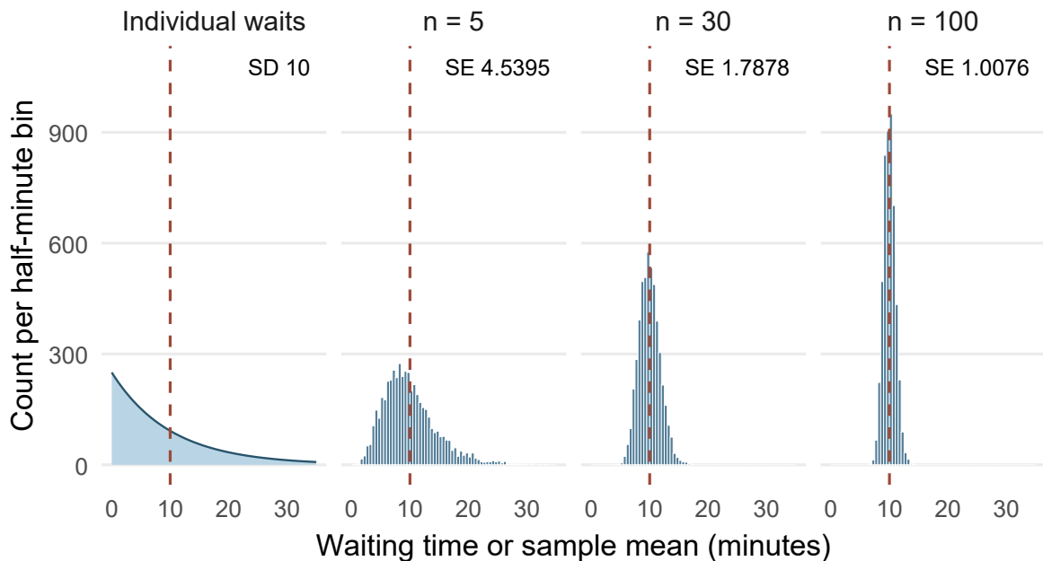
Figure 15: Individual waiting times and simulated sampling distributions of their mean. The first panel shows the exponential model for individual waits, with population mean and SD both 10 minutes, scaled to the counts expected among 5,000 waits. Each other panel contains 5,000 sample means from independent waits at the stated sample size, labelled with their SD, the empirical SE. The dashed line marks the population mean.
