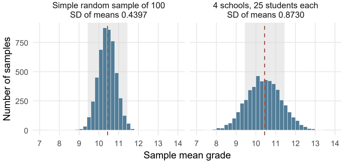
Figure 16: Same sample size, different design. Each panel contains 5,000 means of 100 grades drawn from one invented population of 20,000 students in 100 schools. The dashed line marks the population mean, 10.4397, and the shading the range within one grade point of it.
