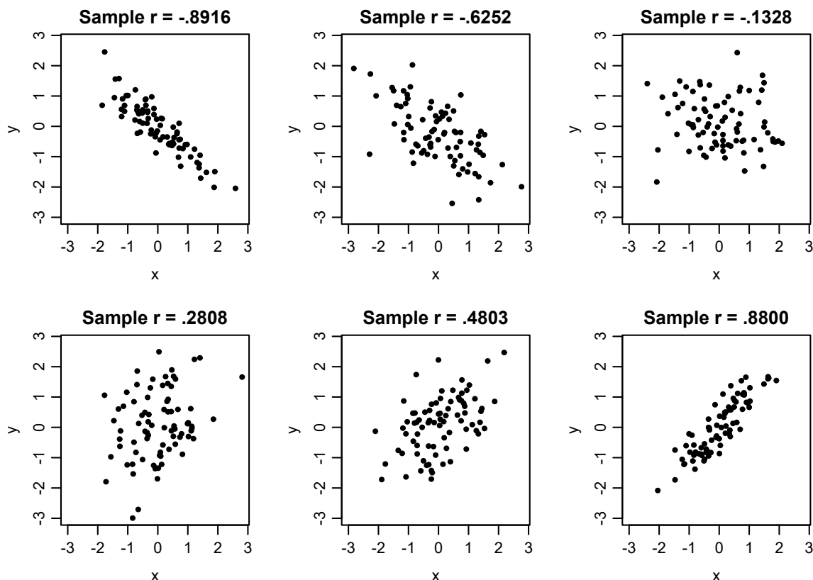
Figure 12: Six simulated scatterplots show different directions and strengths of linear association; labels report the sample correlation of each panel.
