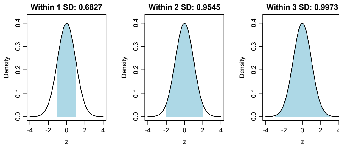
Figure 8: Central Normal probabilities within one, two and three SDs.
