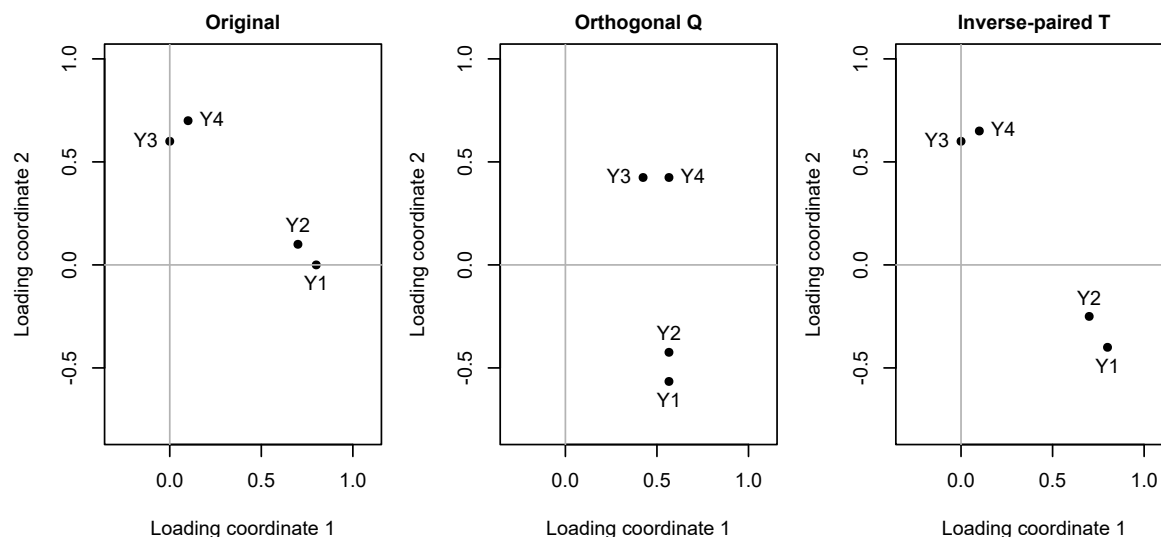
Figure 5: A change of axes in a two-dimensional illustration. These are illustrative loadings, not a second empirical data set.
