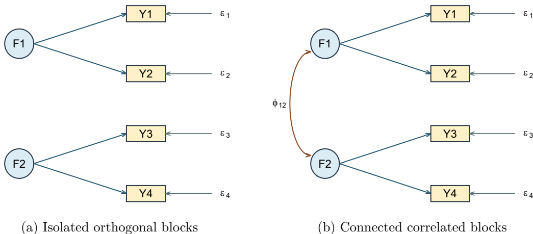
Figure 7: Two-indicator blocks can have the same whole-model count but different recoverability because the covariance edge changes which moments carry loading information.
