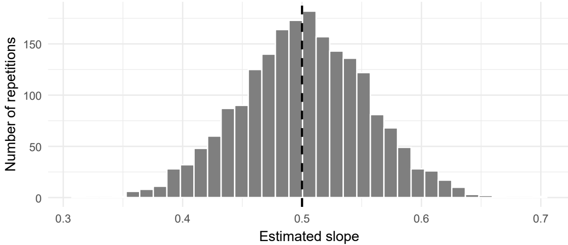
Figure 5: Slopes in 2,000 repetitions of the known process. The vertical reference is the true slope, 0.5.
