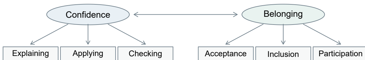
Figure 4: A candidate measurement map for confidence and belonging. Arrows show proposed measurement relationships; the two-headed link represents a possible factor correlation. Indicator-specific variation is omitted from this sketch.
