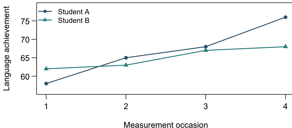
Figure 2: Two invented language-learning trajectories. Equally spaced assessment times allow uneven score changes; the lines join observations rather than represent a fitted growth model.
