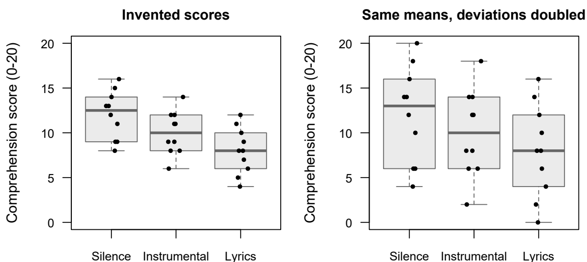
Figure 1: The idea of ANOVA: the same group means with different within-group spread. Left: the thirty invented scores. Right: a constructed version in which every score’s distance from its group mean is doubled, so the group means and counts are unchanged, although the medians that the boxes mark can shift. Boxes show each group’s median and middle half; each point is a student, jittered sideways so that equal scores stay visible.
