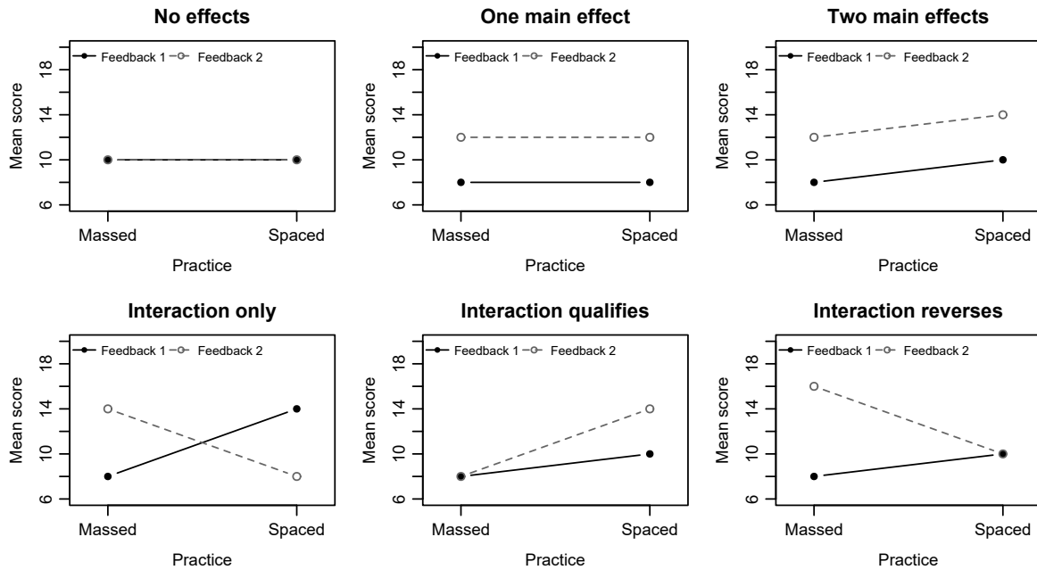
Figure 5: Six schematic patterns of cell means, covering the whole range of main-effect and interaction combinations. The two lines are two levels of a feedback factor; the drawings illustrate averages and changing differences, without significance claims.
