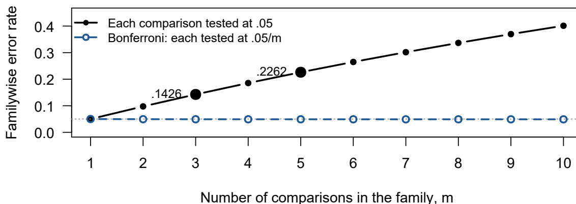
Figure 4: The familywise error rate for m hypothetical independent comparisons whose null hypotheses are all true, each tested at .05 (upper line) or at Bonferroni's .05/m (lower line).
