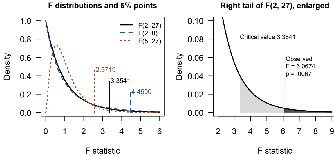
Figure 3: F distributions and the one-way statistic. Left: three F distributions, each indexed by its numerator and denominator df; a vertical mark in each curve's colour and line type, labelled with its value, shows the point beyond which 5% of that distribution lies. Right: the right tail of F(2, 27), enlarged. The shaded areas together are the .05 beyond the critical value 3.3541; the dark area beyond the observed statistic 6.0674 is the p-value, .0067.
