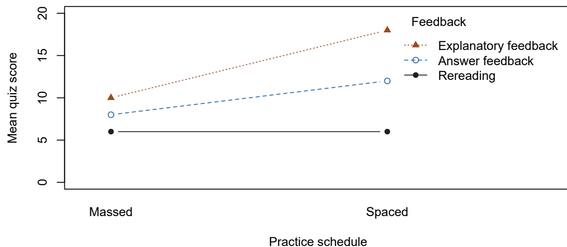
Figure 6: Quiz cell means across practice schedules in the full 3 \times 2 example. Each line joins means of different students; the schedule differences are 0, 4 and 8 points.
