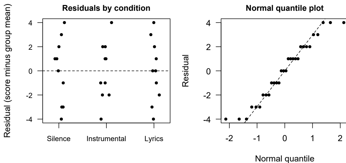
Figure 9: Residuals of the one-way fit to the background-sound scores. Left: each student’s residual, the score minus the group mean, by condition, jittered sideways so that equal values stay visible. Right: the thirty residuals against Normal quantiles, with a reference line.
