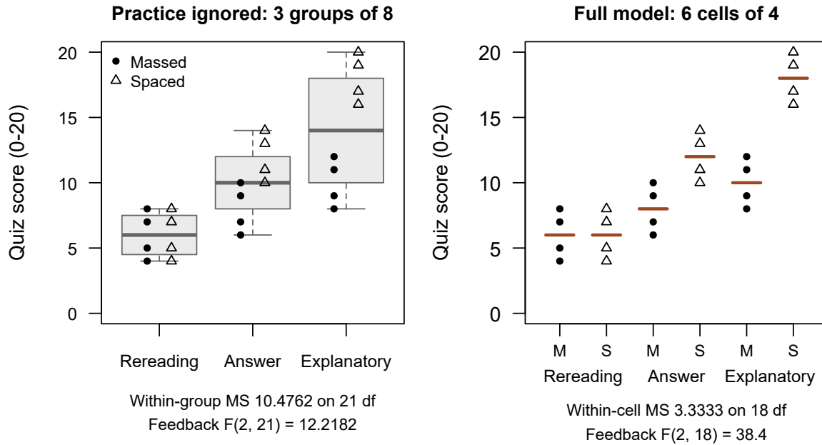
Figure 7: The 24 feedback-by-practice scores analysed two ways. Left: practice is left out, so each feedback condition is one group of eight; filled circles mark Massed and triangles Spaced students. Right: the six cells of the full model, with a bar at each cell mean. Leaving practice out moves the practice and interaction variation into the within-group term.
