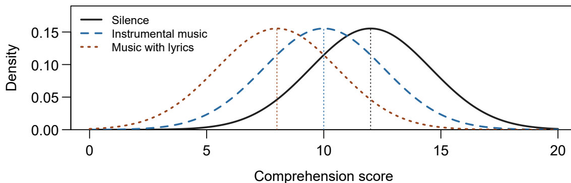
Figure 2: The one-way model for the background-sound study: the scores of each condition vary Normally around that condition's model mean, with one spread common to all three. The curves are drawn at the observed means 12, 10 and 8 with the common SD estimated by the square root of the within-group mean square, 2.5676.
