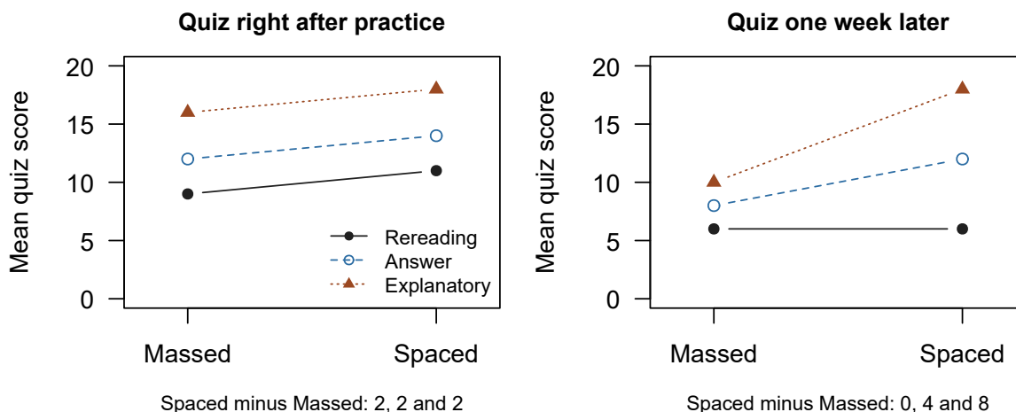
Figure 8: Cell means of the three-way study. Each panel is the feedback-by-practice plot for one quiz timing, with each line joining means of different students. Right after practice the lines are parallel, so Answer's schedule difference minus Rereading's is 0; one week later they fan out, and the same difference of differences is 4. That change across timing is a three-way interaction.
