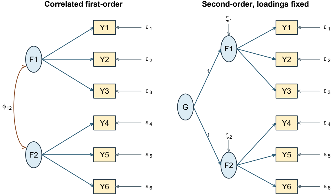
Figure 8: A correlated two-factor model and one constrained second-order reparameterization. The equivalence requires the stated fixed loadings and admissible disturbance variances.
