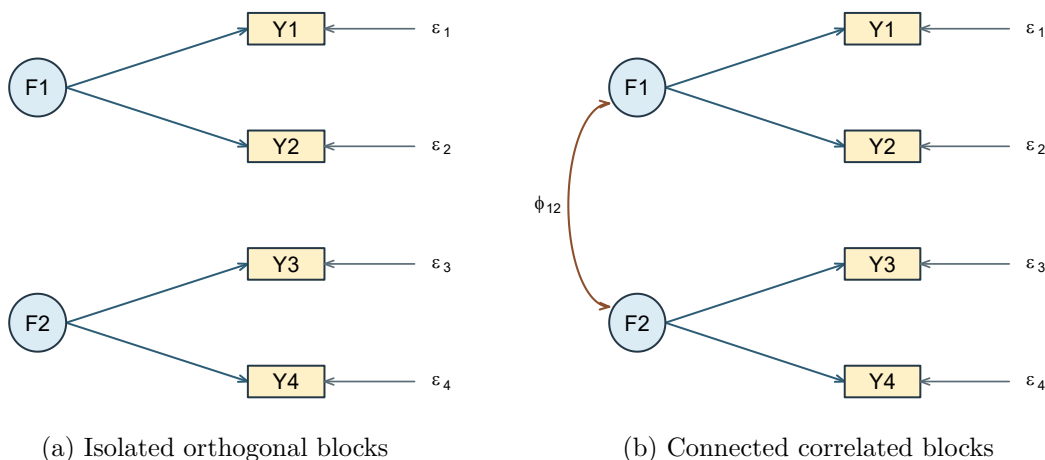
Figure 7: Both two-indicator models have positive nominal degrees of freedom, yet different recoverability. Adding the covariance edge increases the free-parameter count from eight to nine and supplies informative cross-block moments.
