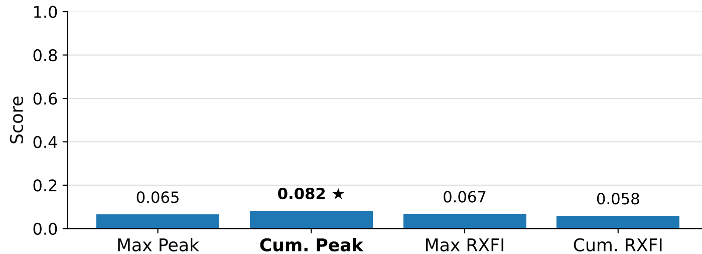
HSS
