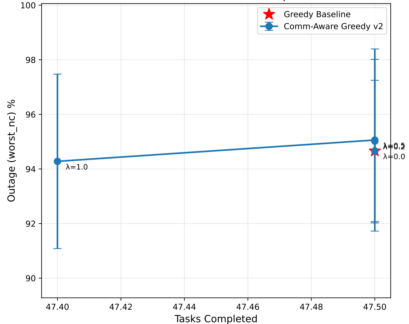
Trade-off Curve: Dual Hotspot
