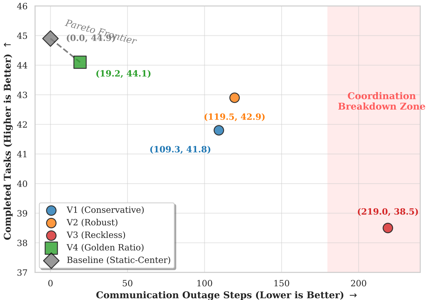
Pareto Analysis: Task Completion vs. Communication Quality
