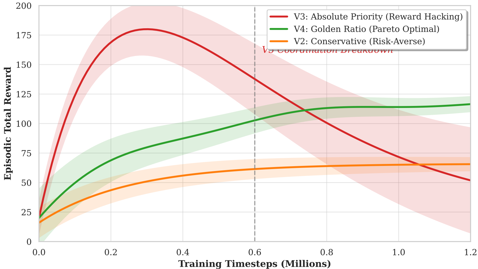
Training Convergence with Dynamic Entropy Decay
