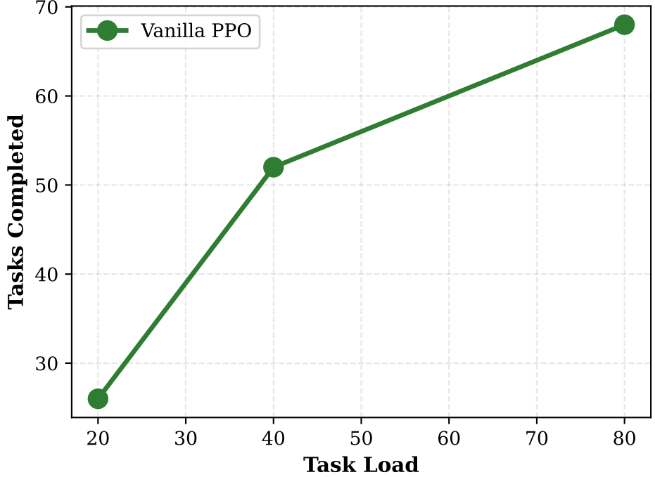
Tasks Completed vs Task Load
