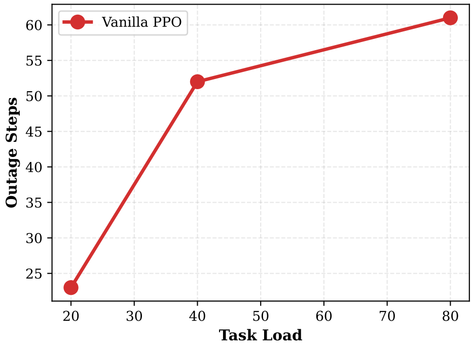
Outage Steps vs Task Load
