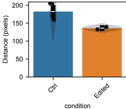
Total Closest-Island Distances
