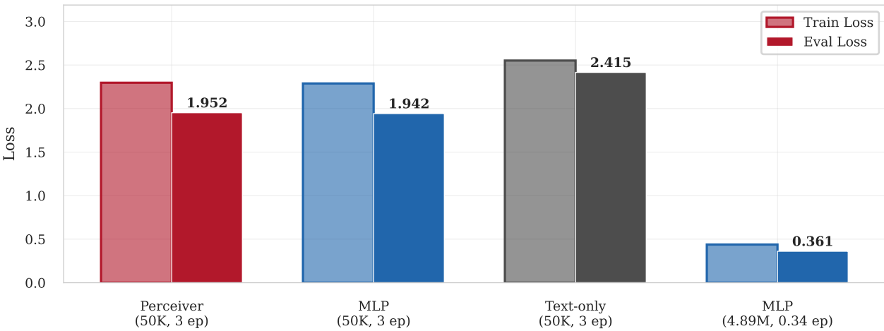
Final Metrics: Approach Comparison
