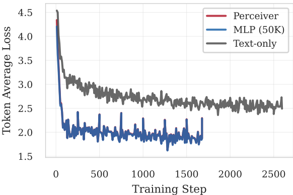
Training Loss by Approach (50K Samples)
