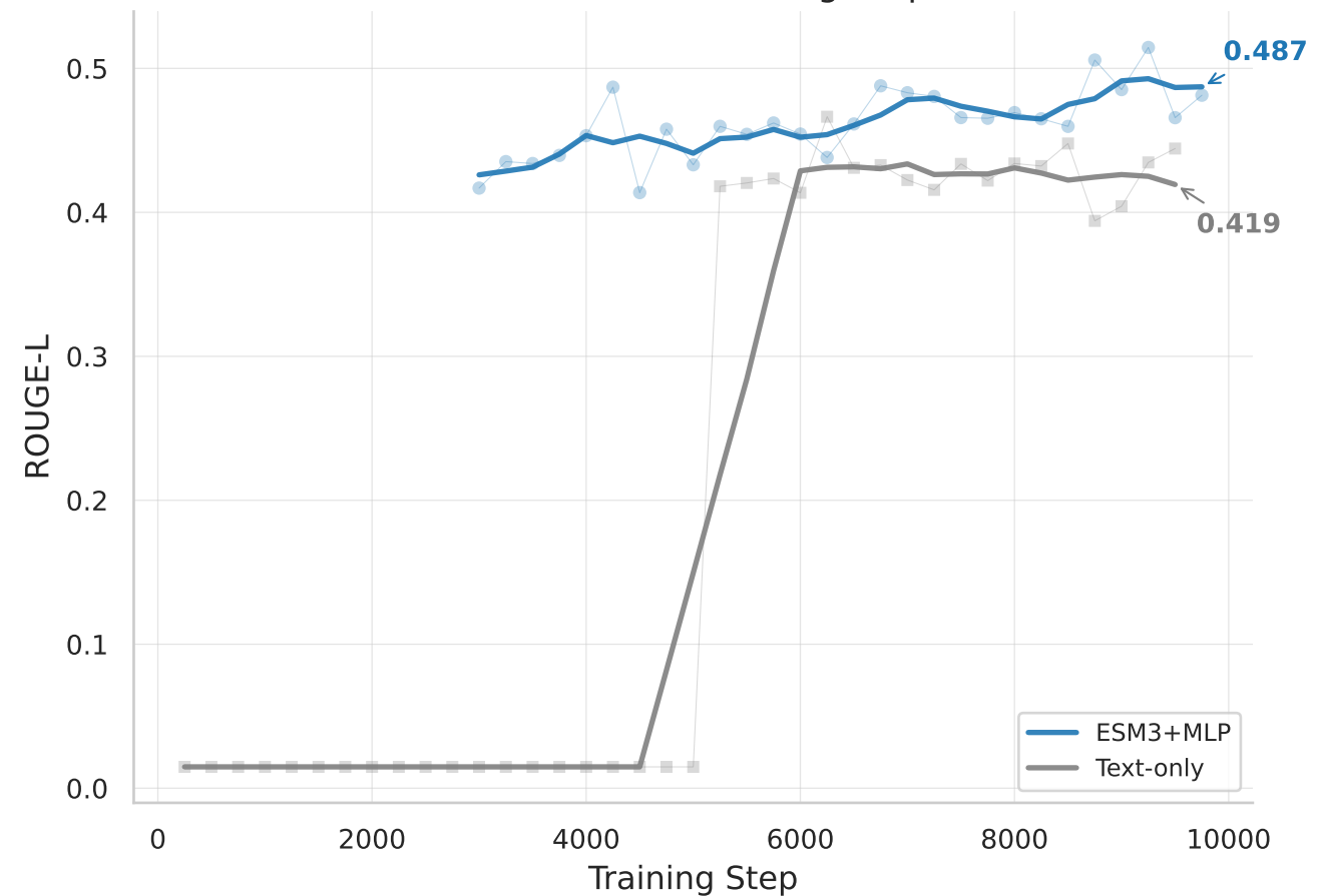
ROUGE-L Over Training Steps
