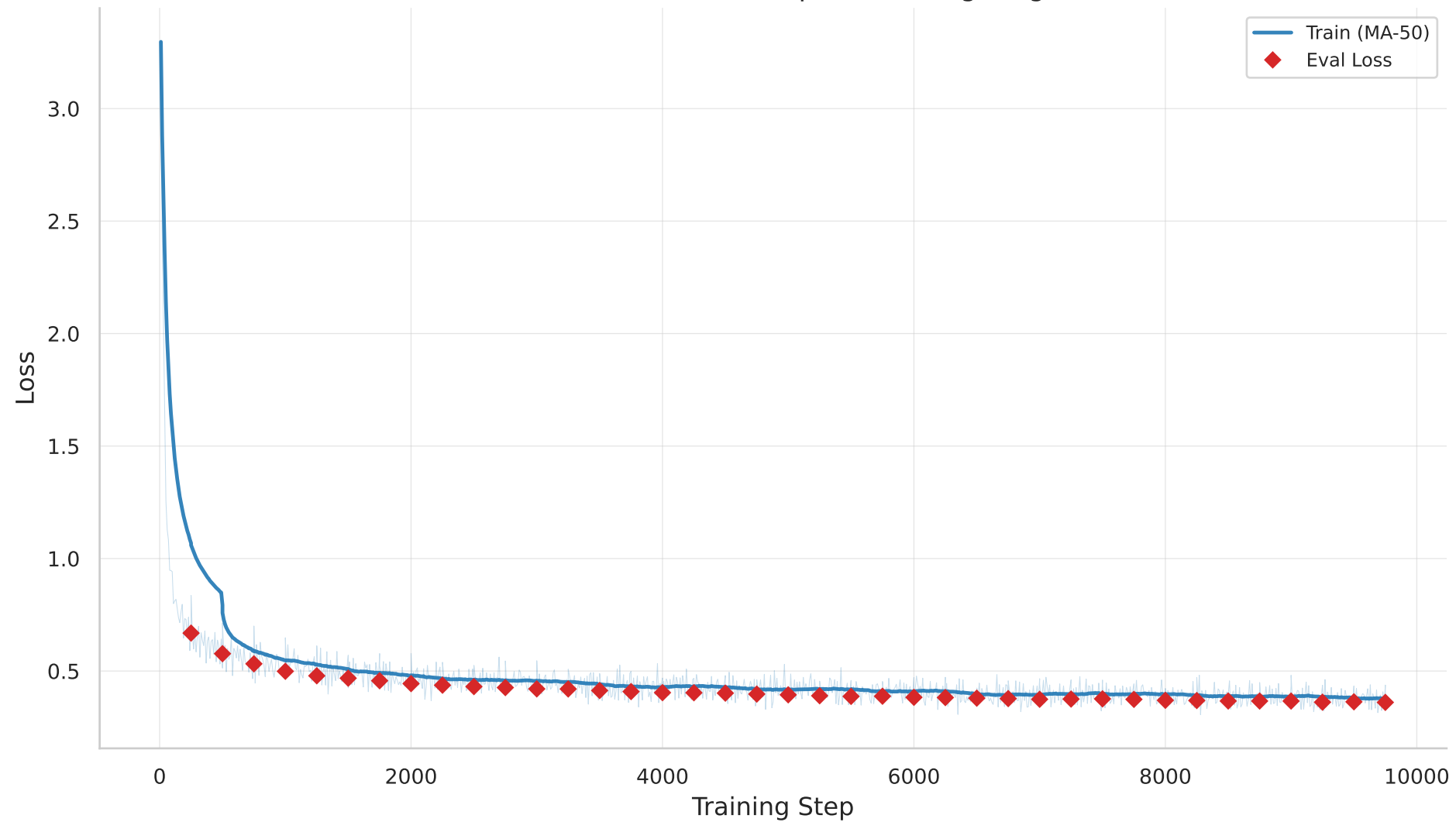
ESM3+MLP on 4.89M Samples: Training Progress
