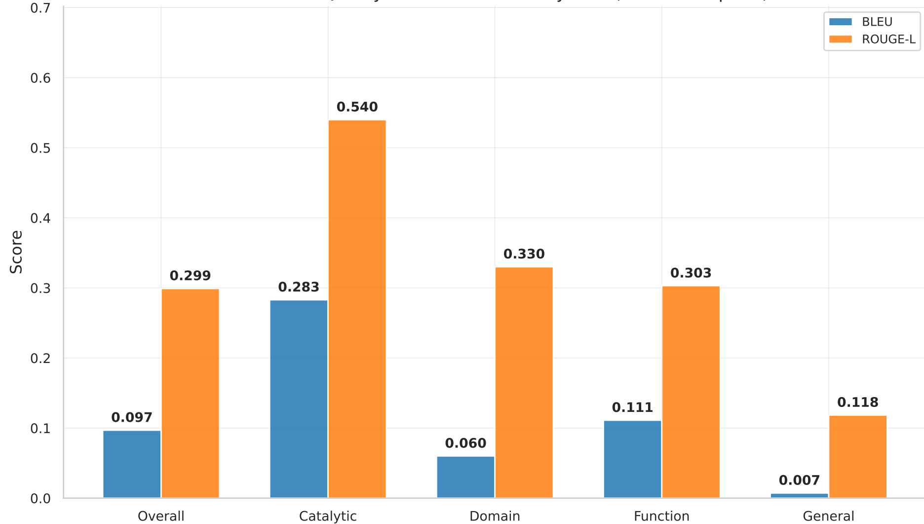
Generation Quality: BLEU & ROUGE-L by Task (Final Checkpoint)
