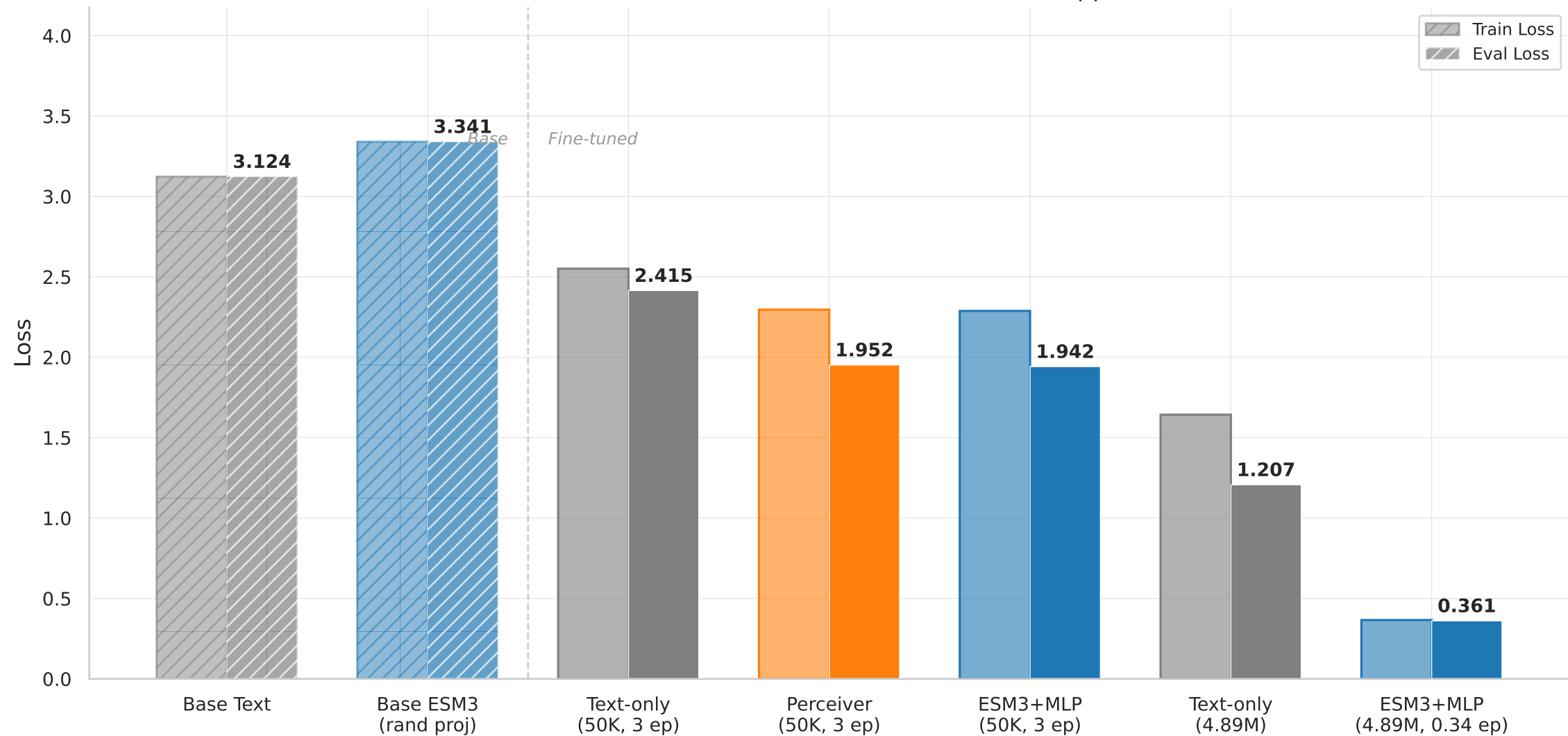
Final Metrics: Base Model Baselines vs Fine-tuned Approaches
