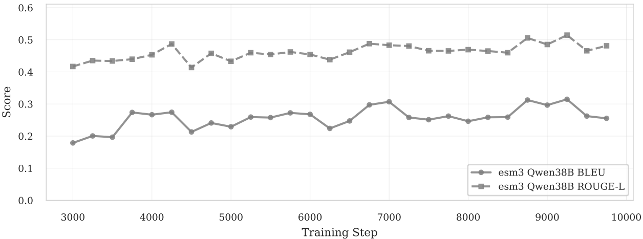
Generation Quality Over Training
