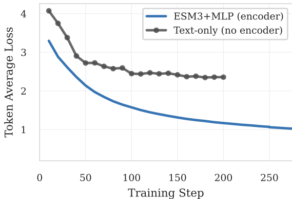
ESM3+MLP vs Text-only on 4.89M Combined Dataset
