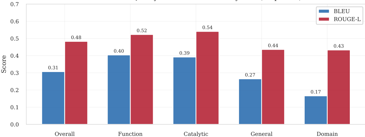
Generation Quality: BLEU & ROUGE-L by Task (Step 7000)
