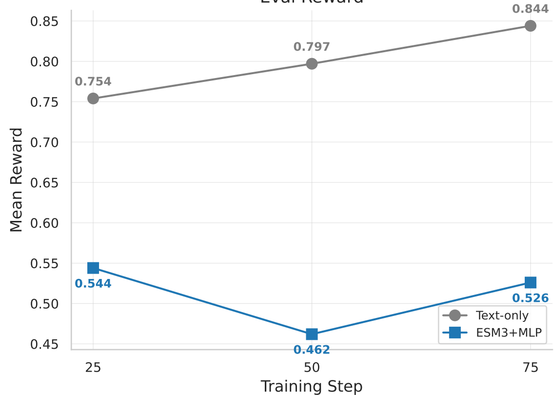
Eval Reward
