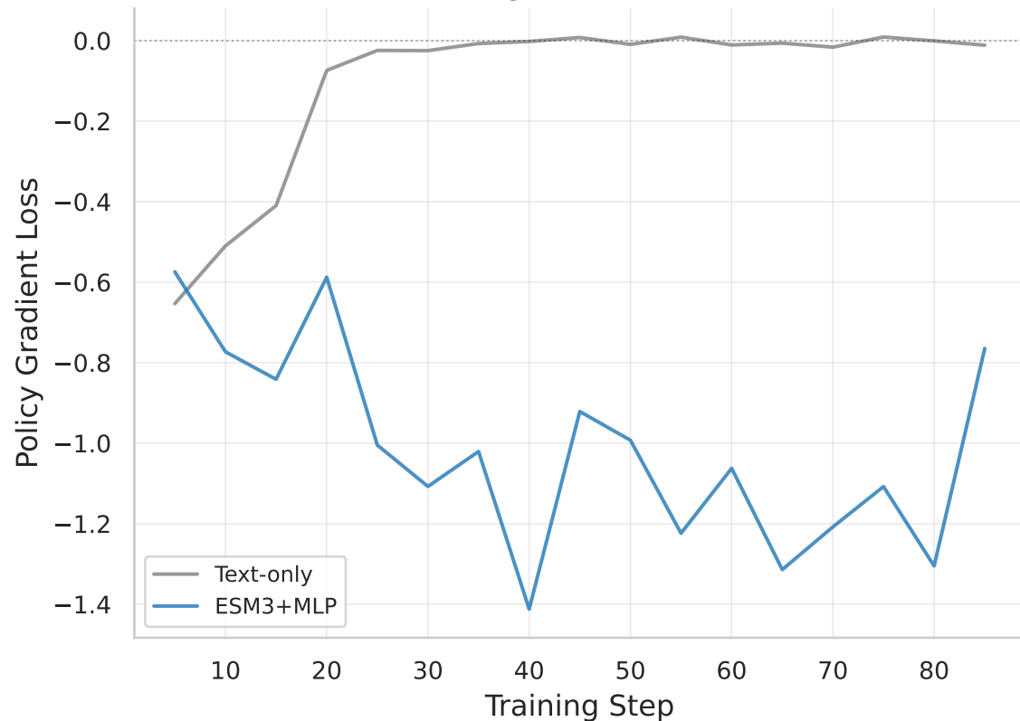
Training Loss (PG Loss)
