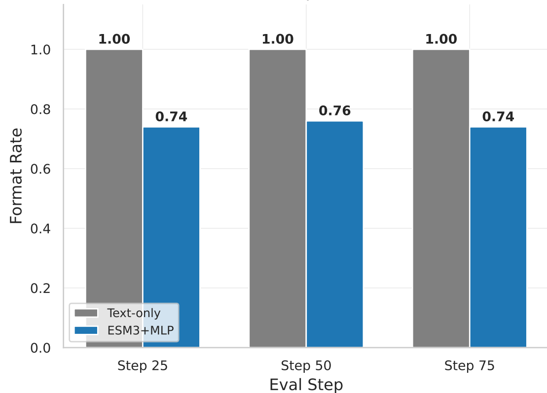
Format Compliance Rate
