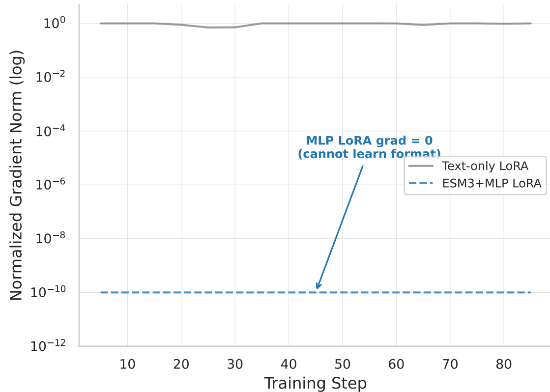
LoRA Gradient Norms
