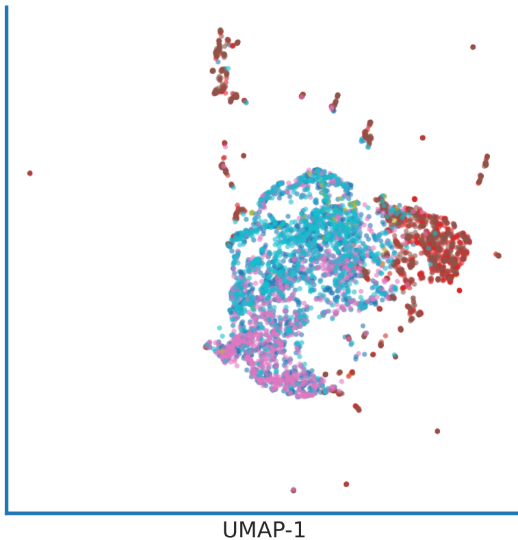
Trained Projector
