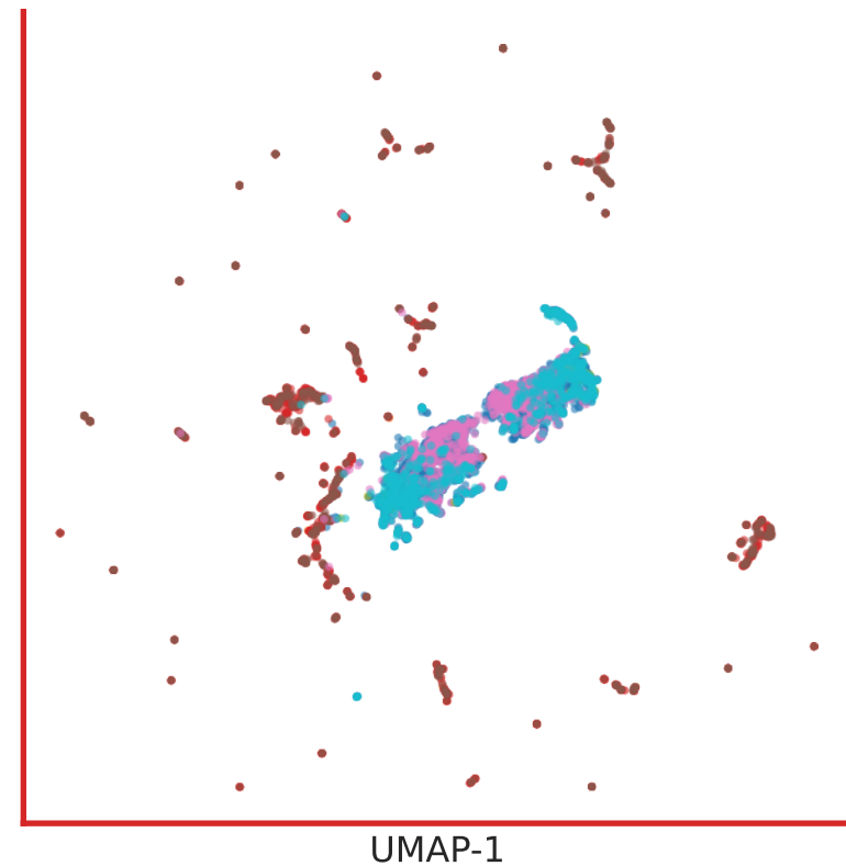
Random Projector
