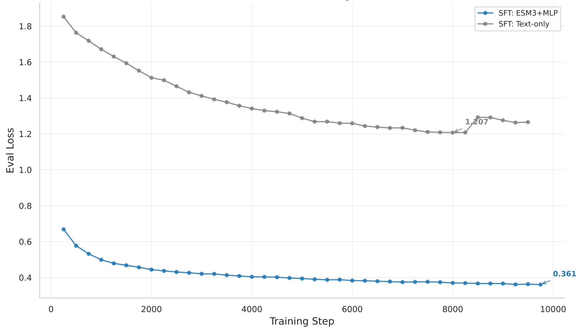
SFT Eval Loss: ESM3+MLP vs Text-only (Qwen3-8B, 4.89M)
