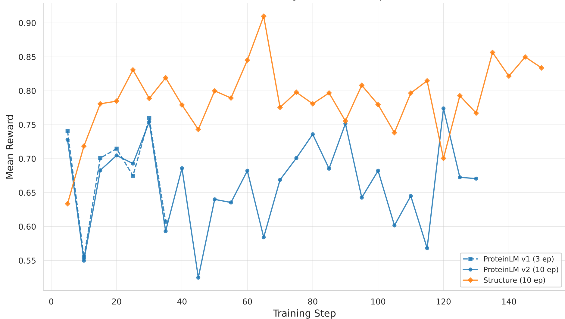
GRPO Training: Reward vs Step
