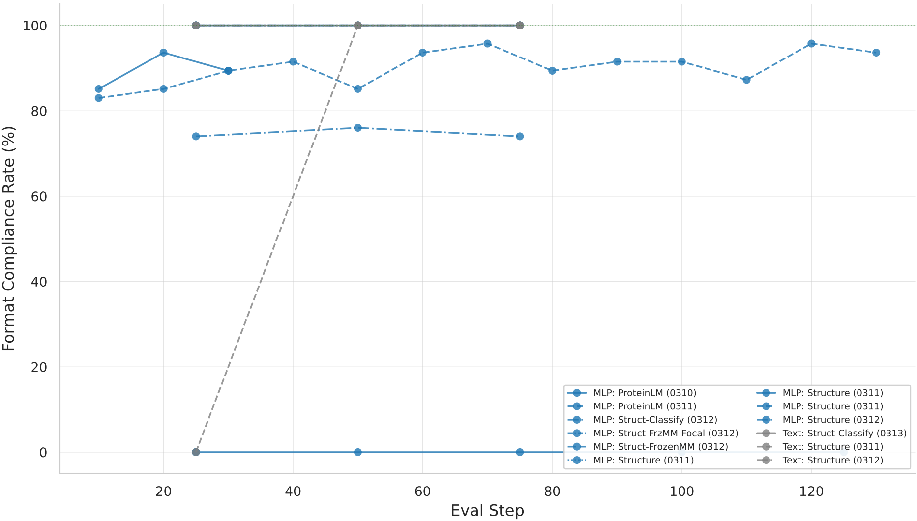
GRPO Format Compliance Over Training
