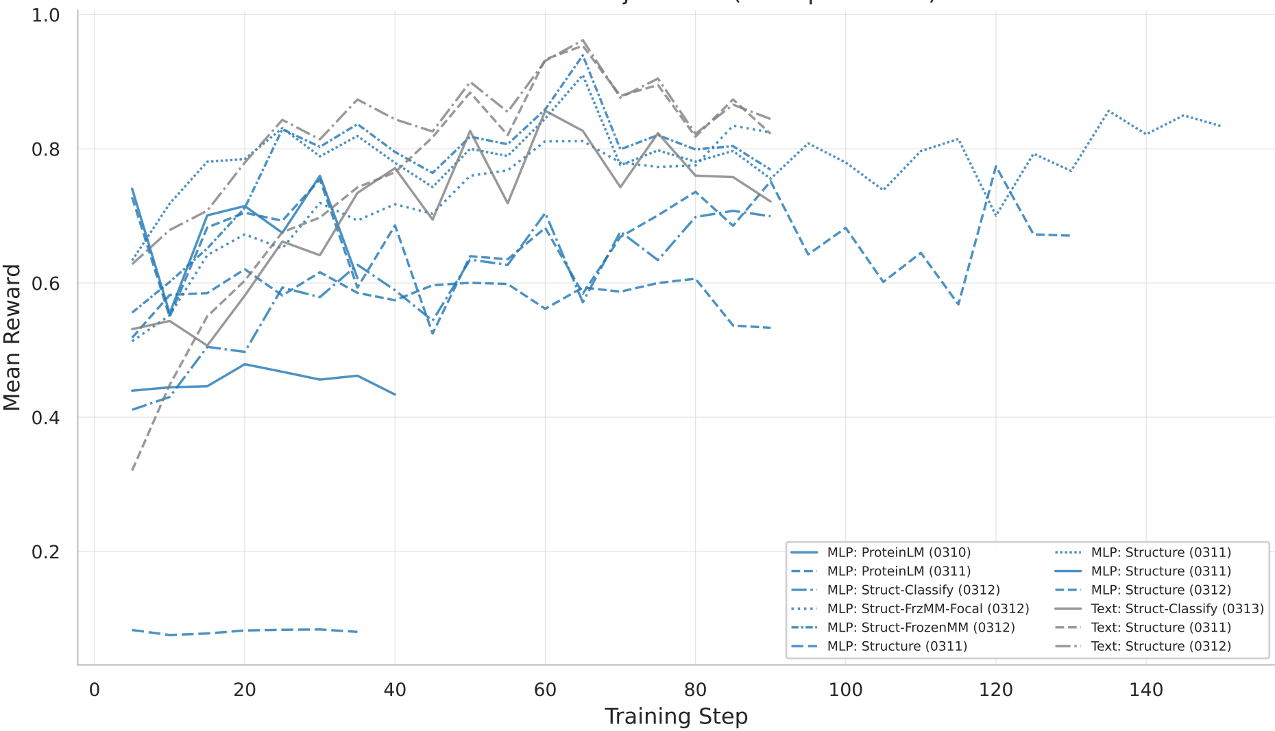
GRPO Reward Trajectories (All Experiments)
