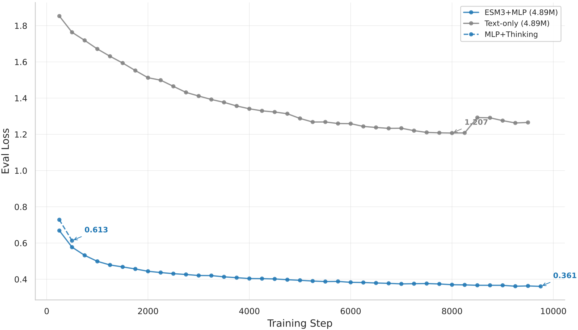
SFT Eval Loss Curves (All Experiments)
