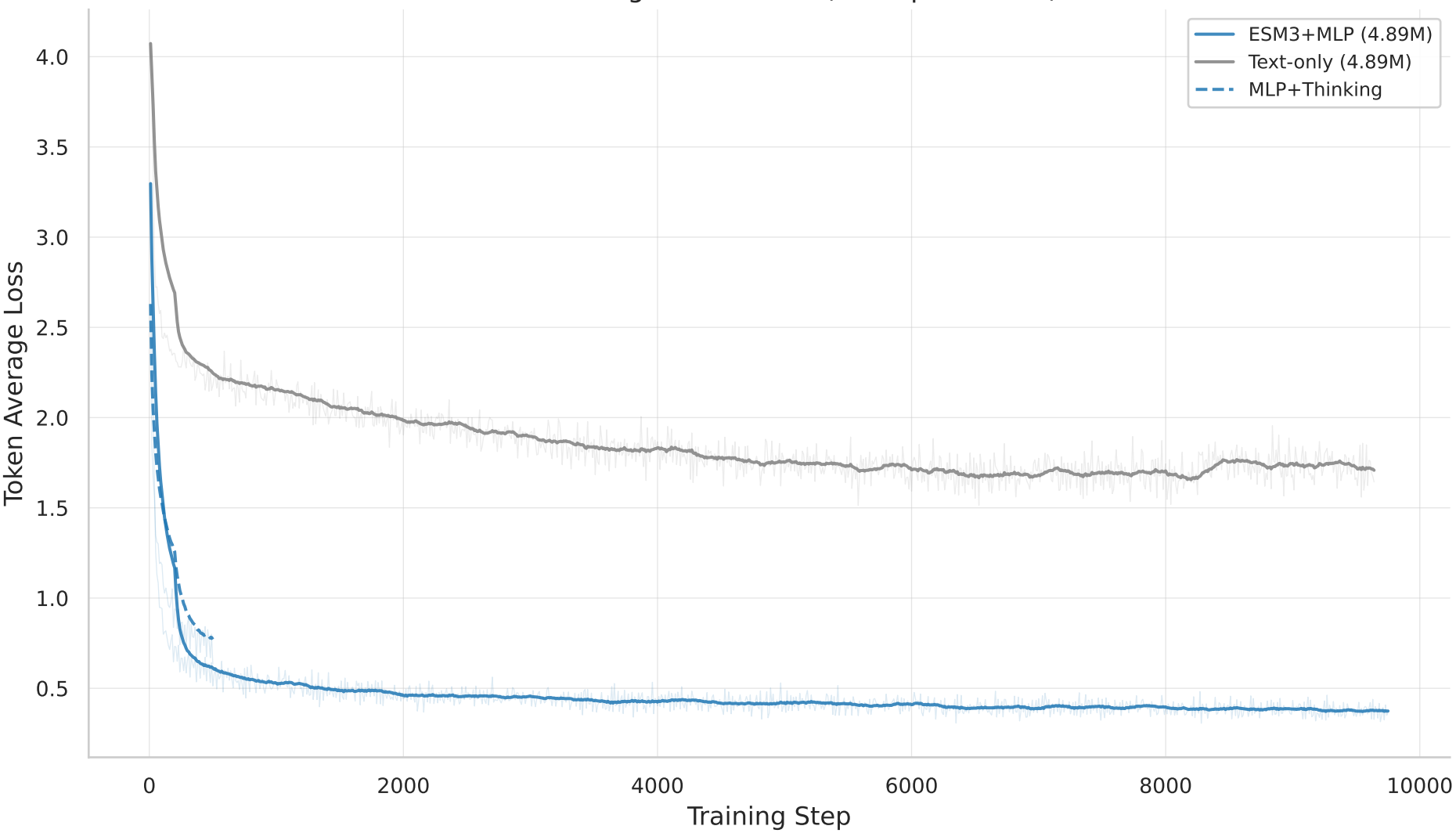
SFT Training Loss Curves (All Experiments)
