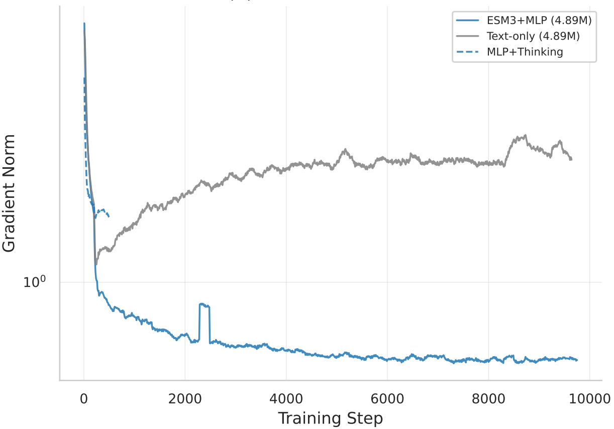
(C) SFT Gradient Norms
