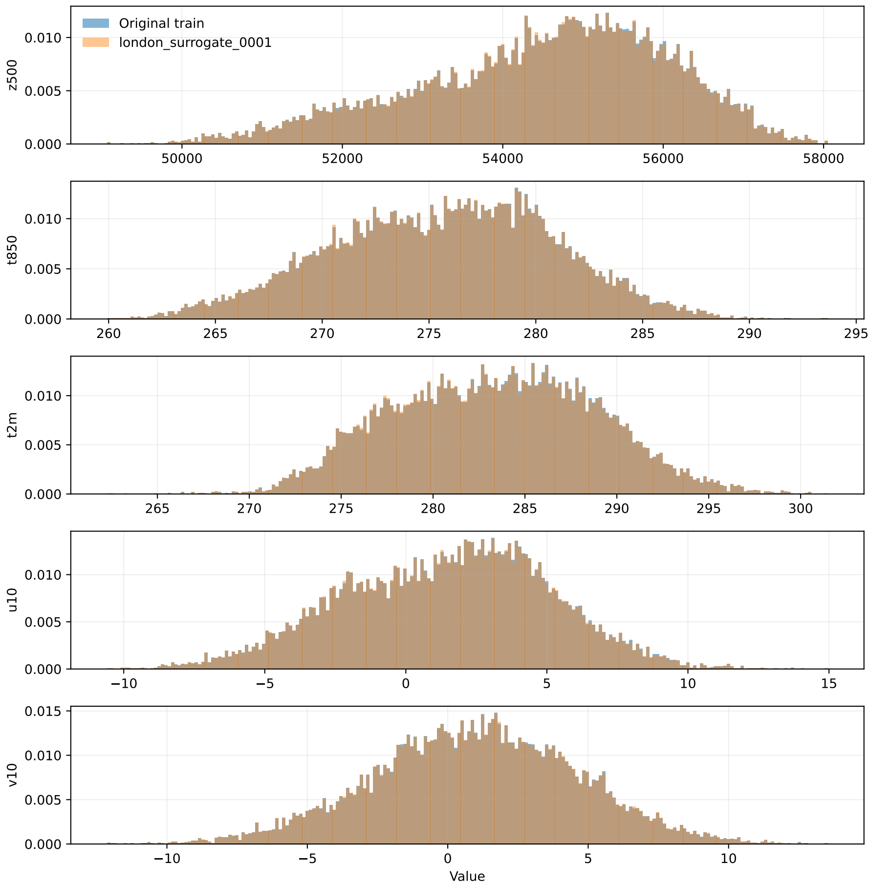
Feature distributions: Original train vs london_surrogate_0001
