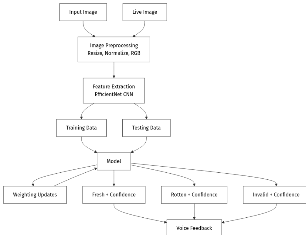
Figure 4.2: QualiVision AI Project Pipeline
