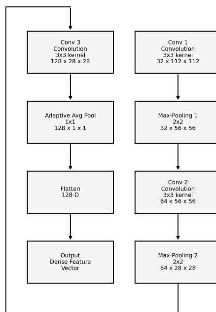
Figure 4.2: CNN Architecture Pipeline
