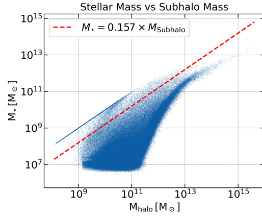
Figure 2.3: Scattered stellar mass vs subhalo mass. The red dashed line indicates a linear relation with a slope of f_b = 0.157 . The expresses a theoretical upper limit for the stellar mass that can be contained in a halo. Here it can be observed that some subhalos host galaxies with stellar mass exceeding this limit.
