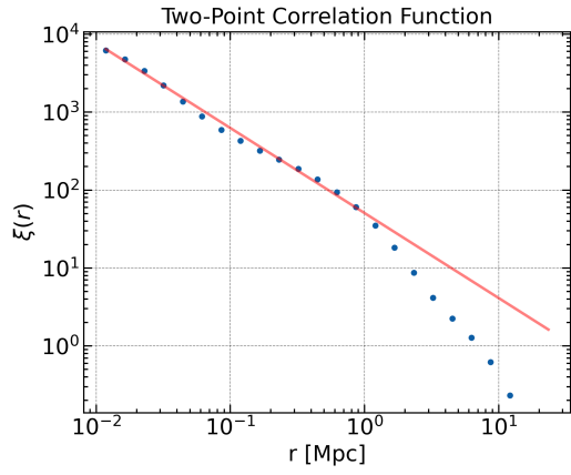
Figure 2.2: Two-point correlation function \xi(r) of subhalos hosting galaxies. The red line indicates a power-law fit to the data points, with parameters r_0 = 36.60 Mpc and \gamma = 1.09 . Deviation from the power-law for r \gtrsim 1 Mpc can be observed.
