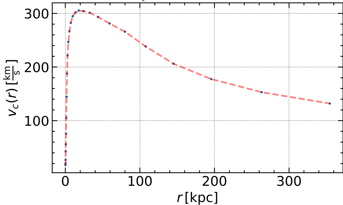
Circular Velocity Profile of Dark Matter Subhalo
