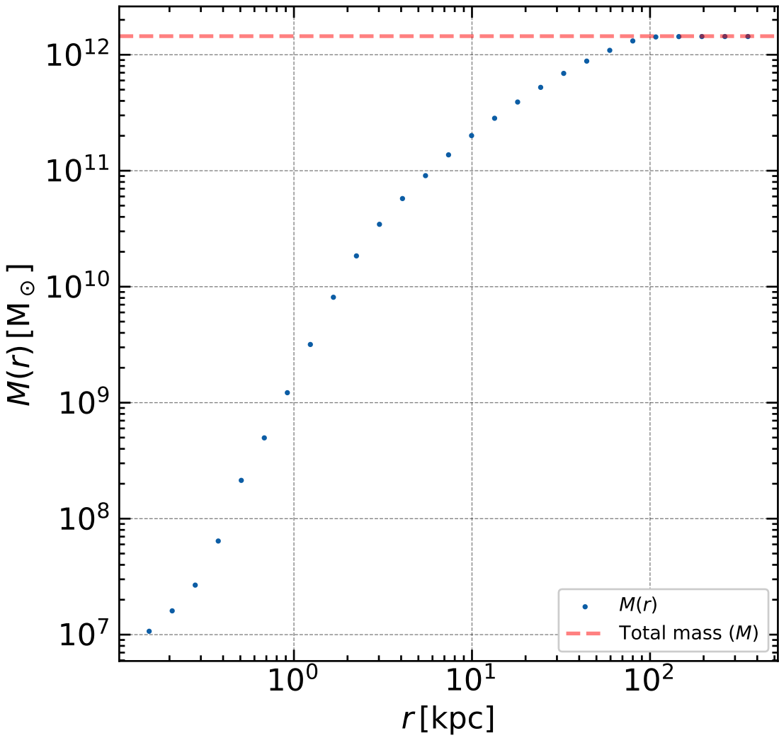
Enclosed Mass Profile
