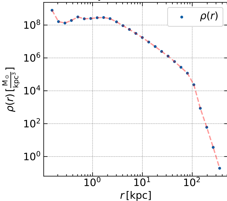
Radial Density Profile of Dark Matter Halo
