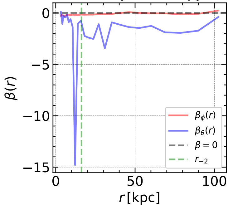
Velocity Anisotropy
