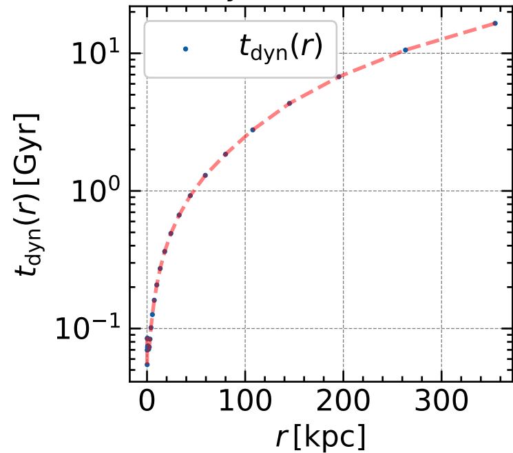
Dynamical Time
