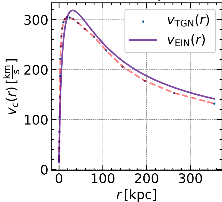
Circular Velocity Profile
