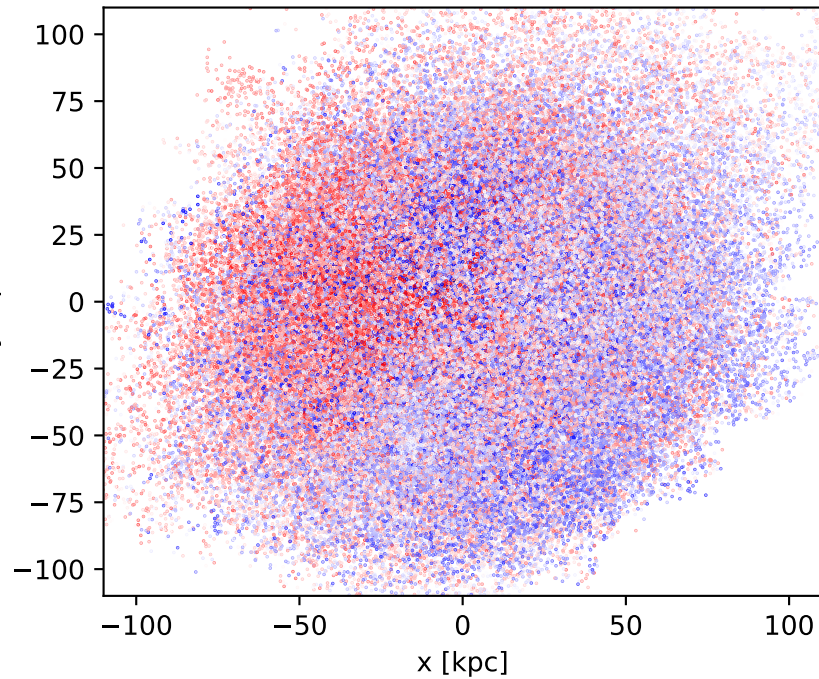
DM distribution in xy-plane
