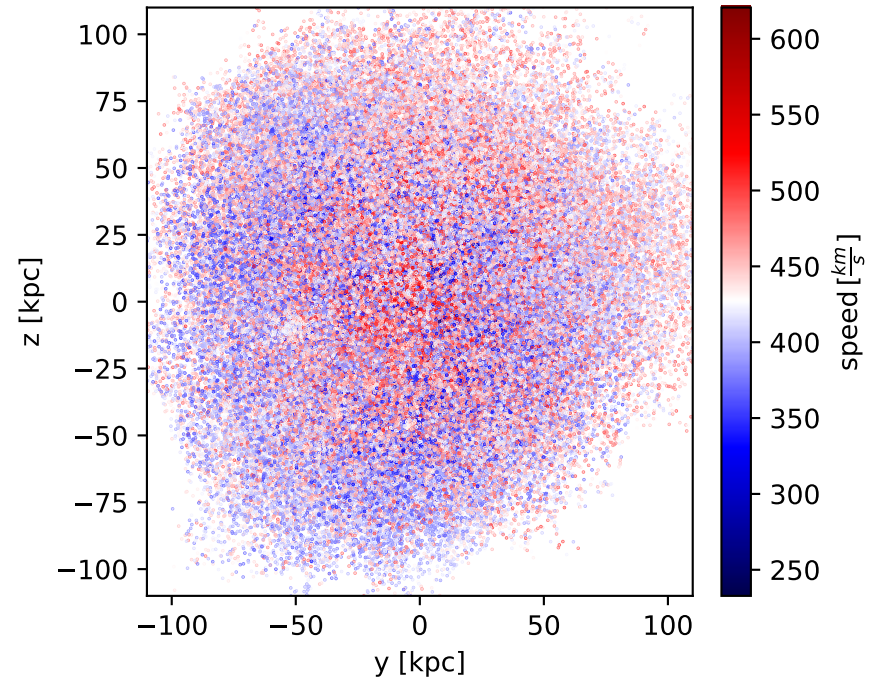
DM distribution in yz-plane
