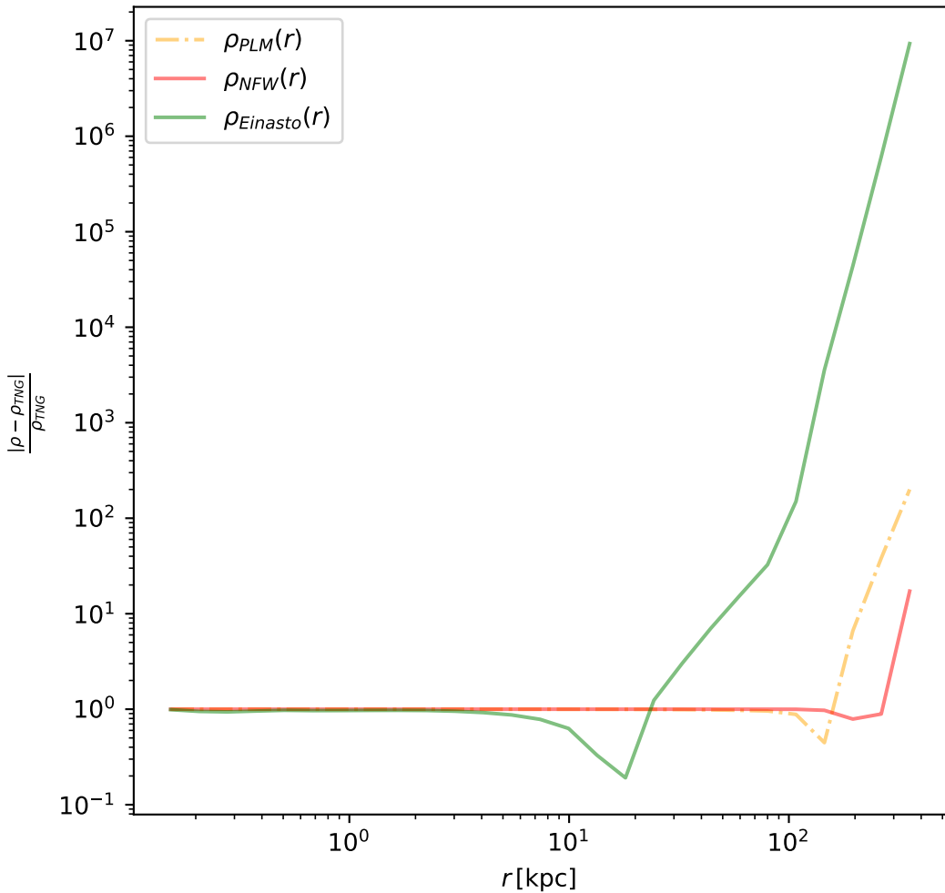
Relative Error galpy calculation
